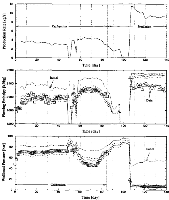
Figure 8. Calibration and prediction of flowing enthalpy and wellhead pressure. The top panel shows the prescribed production rate. Squares are measured data used for calibration. Triangles are measured data used for validation. The dash-dotted lines are the model results with the initial parameter set (see Table 4). Simulation results based on the estimated parameter set are shown as solid lines. Error bands (dashed lines) are calculated using linear uncertainty propagation analysis.
