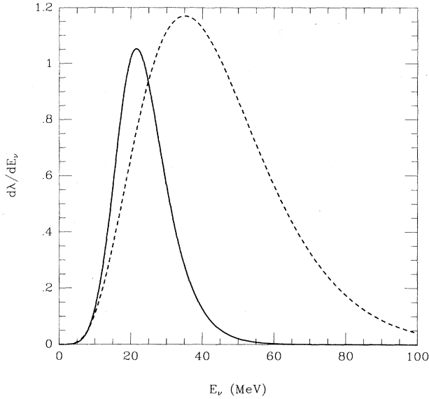
FIG. 1. Differential \bar{\nu}_e capture rate on proton with respect to \bar{\nu}_e energy. The solid line corresponds to the original \bar{\nu}_e energy distribution at TPB=6 s. The dashed line is obtained when the \bar{\nu}_e assume the same energy distribution as the \bar{\nu}_\mu at TPB=6 s.
