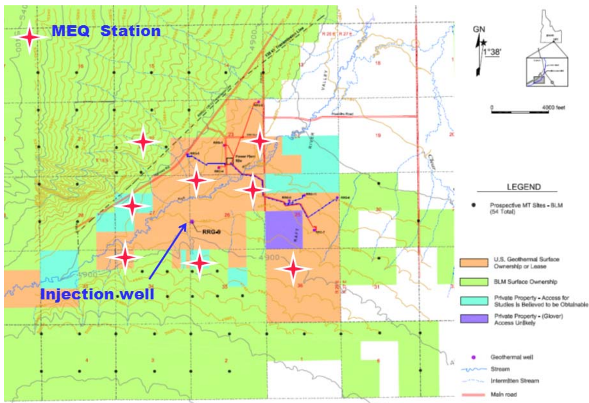
Figure 4-2. Example Local Seismic Array
