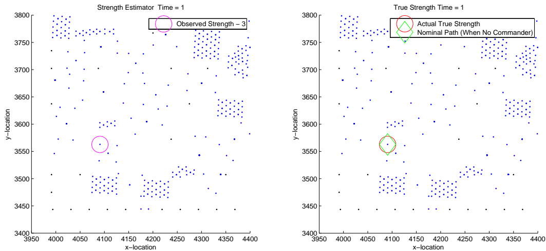
Figure 3.1: Deterministic Movement, Initial Time-Step
