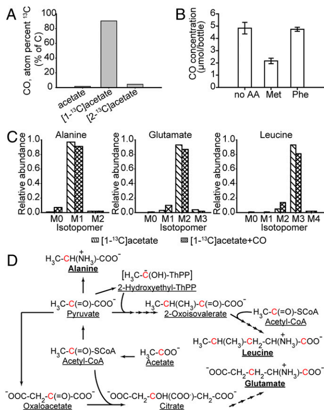
Fig. 4. CO released and incorporated by strain 195. (A) 13 CO was dominant in the cultures amended with [1- 13 C]acetate, but not in cultures amended with either unlabeled or [2- 13 C]acetate. (B) CO quantified in 195 cultures grown in the presence of methionine (Met), no amino acid (no AA), or phenylalanine (Phe). (C) Relative abundance of isotopomers for alanine, glutamate and leucine in strain 195 cultures grown on [1- 13 C]acetate with or without unlabeled CO. (D) Biosynthesis of alanine, glutamate and leucine from acetyl-CoA. ThPP, thiamine diphosphate.
