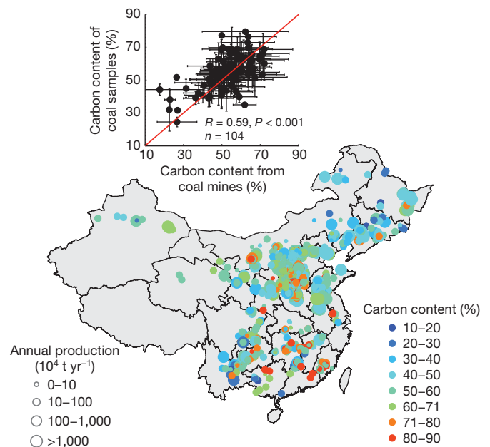
Figure 1 | Total carbon content and production of coal mines. The inset shows the comparison between carbon content from 602 coal samples and 4,243 coal mines ( R = 0.59 , P < 0.001 , n = 104 ). Each dot in the inset indicates the average of carbon content from 602 coal samples and 4,243 coal mines in the same 1° by 1° grid. The nearly one-to-one correlation indicates that samples and mines capture the same spatial variability of coal carbon content across China.
