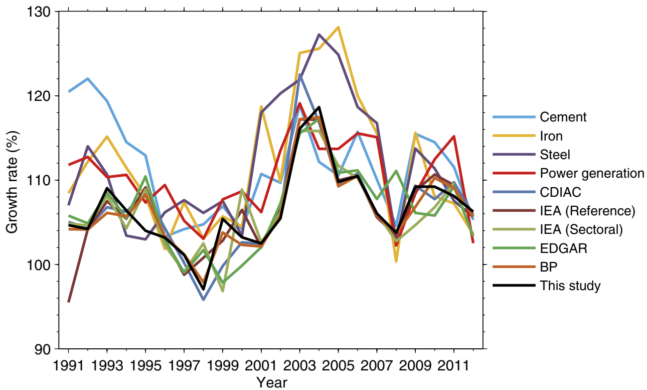
Extended Data Figure 5 | Growth rate of carbon emissions, based upon BP, EDGAR, IEA and calculations in this study, and industrial products. Industrial products comprise the production of cement, iron, steel and power
