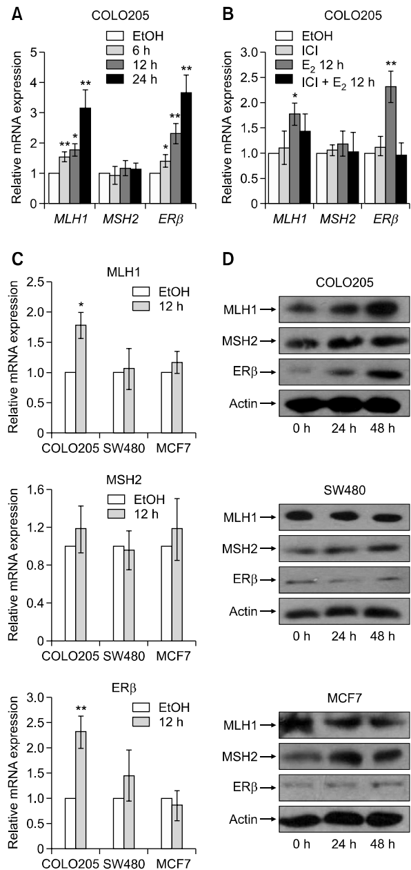
Figure 3. Effects of Estrogen ( E_2 ) on the expression of MLH1 , MSH2 and ER- \beta mRNA. MLH1 and ER- \beta mRNA determined by RT-qPCR in COLO205 cells (A) treated with EtOH or 10^{-9} M of E_2 for 0 h, 6 h, 12 h and 24 h. MLH1 and ER- \beta mRNA determined by RT-qPCR in COLO205 cells (B) pre-treated with estrogen antagonist ICI 182,780 followed by EtOH or 10^{-9} M of E_2 for 0 h and 12 h. Effects of E_2 on MLH1 , MSH2 , and ER- \beta mRNA (C) measured by RT-qPCR in COLO205, SW480, and MCF7 cells. Cells were treated with EtOH, 10^{-10} and 10^{-9} M of E_2 for 12 h. Mean \pm SD from 3 independent experiments. Significant differences between treated group versus EtOH control were calculated by ANOVA (* P < 0.05 and ** P < 0.01 ). Effects of E_2 on protein level expression (D) of MLH1 , MSH2 and ER- \beta in COLO205, SW480, and MCF7 cells.
