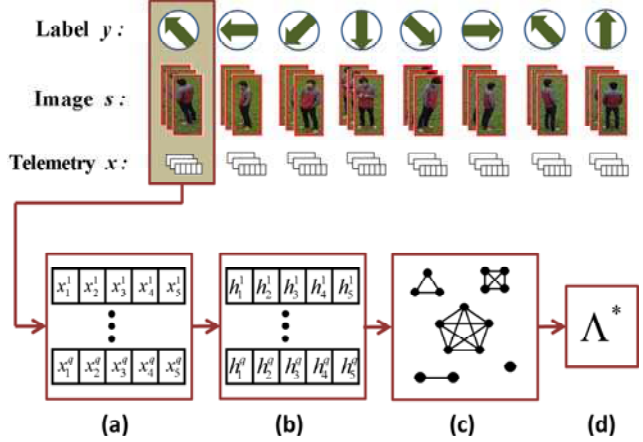
Figure 3: Training Process: The inputs is a set of image patches s from a given label (body orientation) y \in \{y_1, \dots, y_8\} , where each patch is tagged with a set of telemtry data x . The training process involves: a) Collecting a set of telemtry data for each label, b) Obtaining the latent state for each sensor reading, c) exploiting the most significant features using LDCRF and d) output a set of parameters \Lambda^* = \{\lambda^1, \dots, \lambda^5\} , where each \lambda^n is a set of optimal parameters from the n^{th} order interaction.
