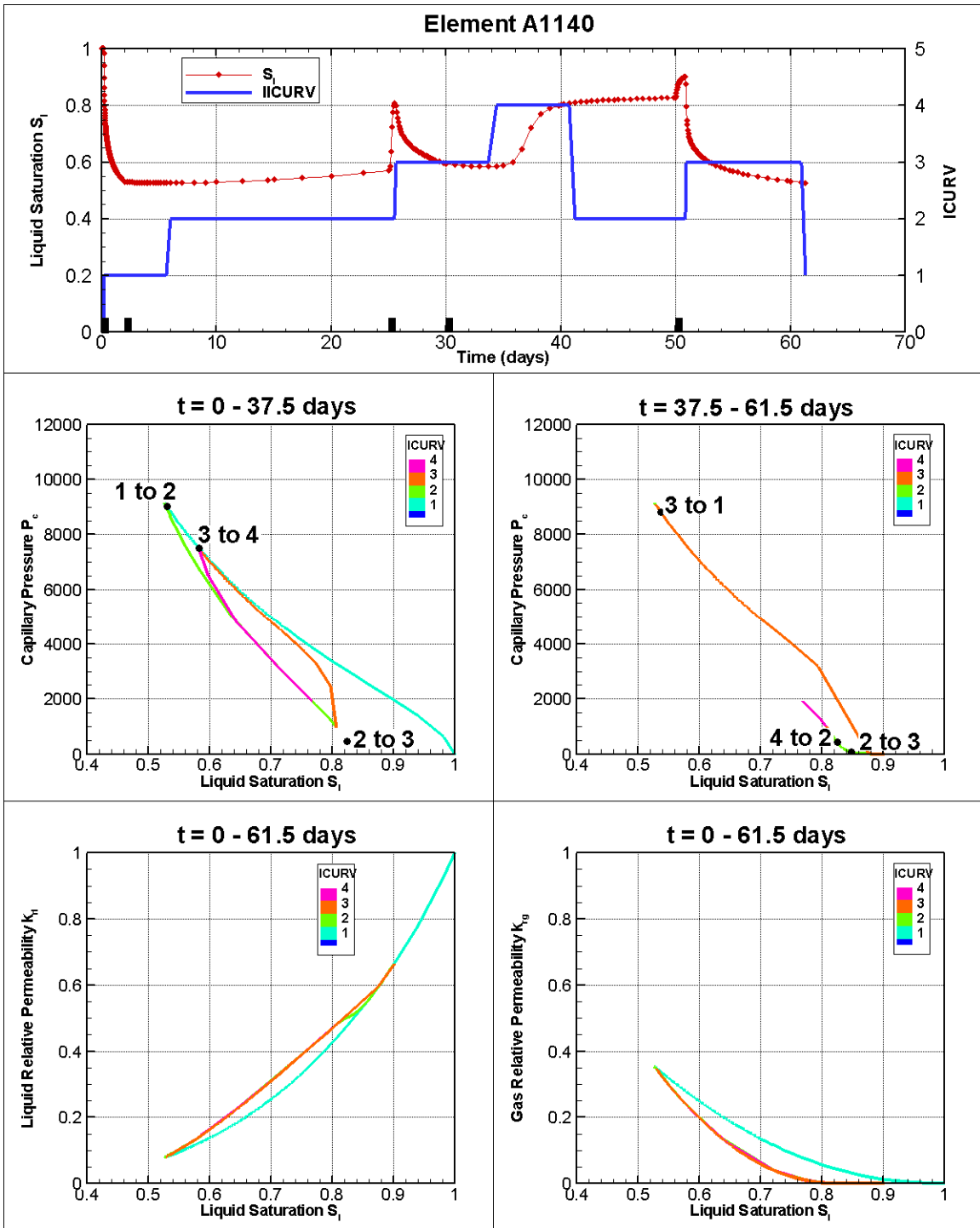
Figure 9. Top: time-variation of liquid saturation and capillary-pressure-curve branch (ICURV) for element A1140. The start of each injection step is marked by a black bar. Middle: capillary pressure versus liquid saturation at element A1140. The plot is divided into two parts, based on time, to enable the different branches of the capillary pressure curve to be seen more easily. The branch switches are marked by black dots, with ICURV for each switch labelled. Bottom: relative permeability versus liquid saturation at element A1140. Branches 2, 3, and 4 all overlie one another.
