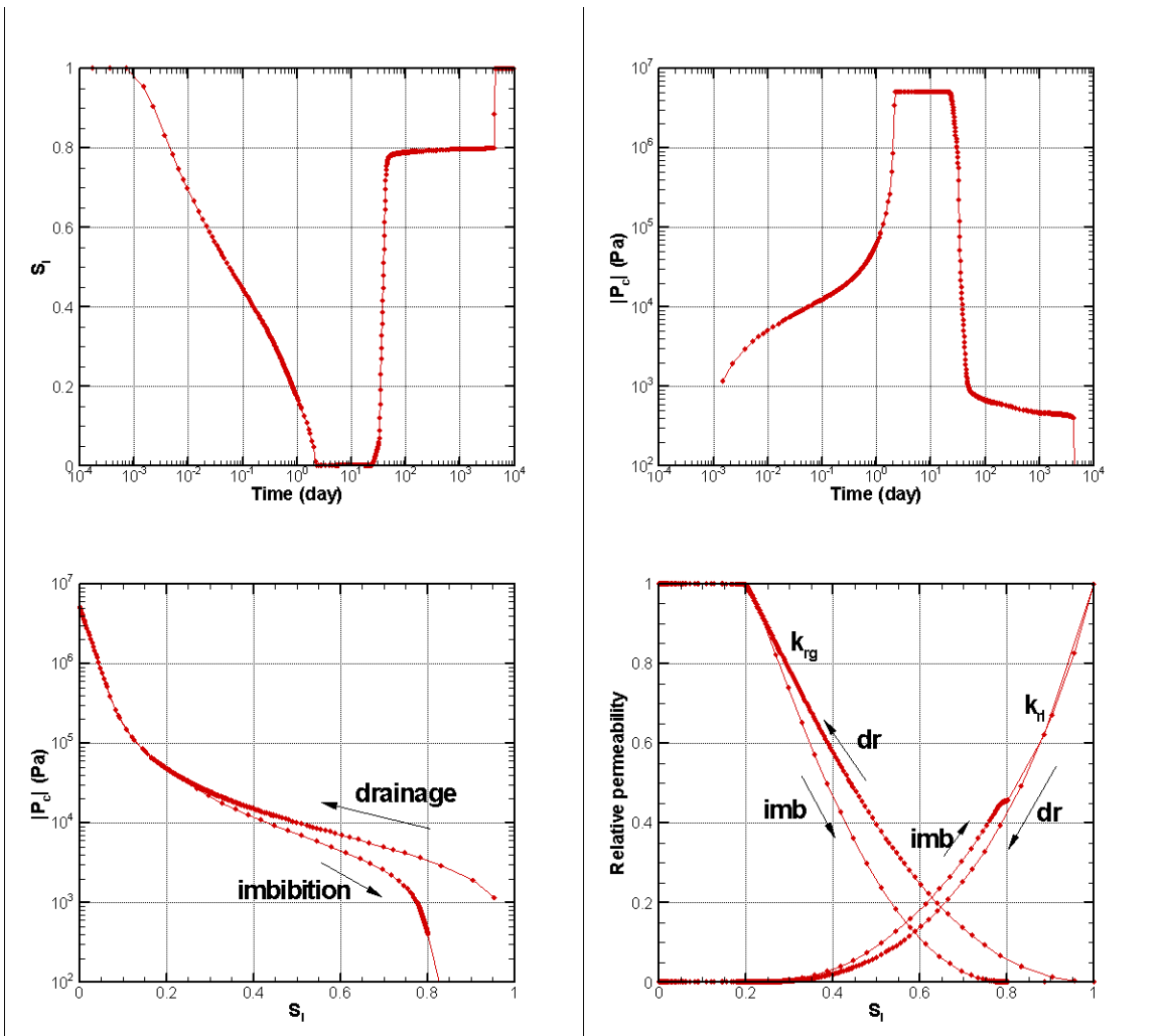
Figure 4. Characteristic curve branches followed for the injection element for Case h203t, in which a large amount of CO 2 is injected for 5 days, followed by 100 years of redistribution.
