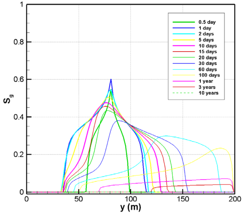
Figure 5. Profiles of S_g versus distance along the model for various times for cases with a small amount of \text{CO}_2 injected for 1 day: j203t (with hysteresis, top) and d203t (no hysteresis, bottom). The injection element is located at y = 81 m. For the hysteretic case, S_{gr}^{\Delta} at 100 days is also shown.
