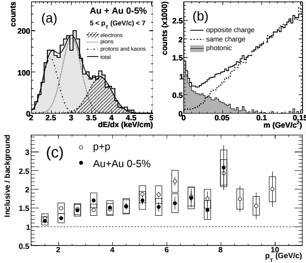
FIG. 1: (a) dE/dx projections for 5 < p_T (\text{GeV}/c) < 7 in central Au+Au events after EMC and SMD cuts. The lines are Gaussian fits for p+K , \pi , and electron yields. (b) Invariant e^+e^- mass spectrum. (c) Ratio of inclusive and background electron yield vs. p_T for p+p and Au+Au collisions. Vertical bars are statistical errors, boxes are systematic uncertainties.
