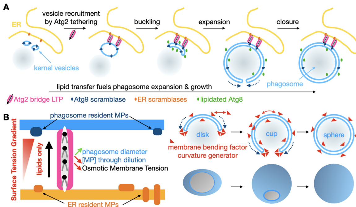
Figure 2. Factors influencing fast bulk lipid transfer through bridge LTPs. A: Autophagosome formation and growth. A phagosome initiates from small vesicles containing scramblase Atg9. Following their Atg2-mediated tethering to the ER and acquisition of lipidated Atg8, bulk glycerophospholipid transfer through Atg2 fuels rapid expansion of these vesicles. B: Effects of vesicle growth on membrane protein (MP) concentration and osmotic membrane tension (OMT). A LTP bridge selectively transfers some lipids but excludes proteins. Local membrane protein concentration and membrane curvature affects surface tension. A gradient of surface tension between donor and acceptor membrane initially drives lipid transfer at rates compatible with phagosome expansion in vivo .
