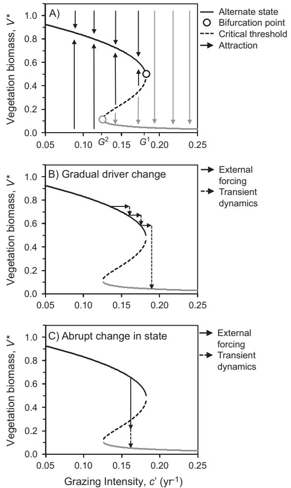
FIG. 2. (A) A fold bifurcation, with two alternative states: a high biomass state (the upper, solid black line) and the a low biomass state (the lower, solid gray line). The two alternative states are attractors to which the system tends to converge. Arrows show the trajectory of the ecosystem for different initial conditions. The unstable equilibria (the dotted line), marks the boundaries of the two alternative states. At this boundary, small changes in state can force the system to the upper or lower state. The point G^1 is a bifurcation point, where the system goes from both the lower and upper state being stable, to only the lower state being stable. The system will start to transition to the upper state if the driver variable is reduced to the second bifurcation point, G^2 . (B and C) Different types of transitions from one alternative state to another. In both panels, the solid arrows represent changes in driver variables, and dashed arrows show transient dynamics. In panel B, the driver variable increases gradually until exceeding a bifurcation point. In panel C, an event alters the state variable, bringing it below a critical threshold. This specific fold bifurcation is generated using the default parameters of the model (Appendix S1).
