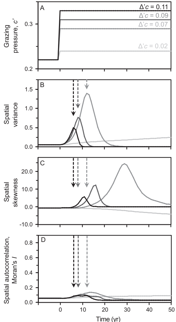
FIG. 10. Changes in (B) spatial variance, (C) skewness, and (D) auto-correlation (lag + 1) over time in response to grazing press intensities (A) of \Delta c' = 0.02 (light gray), \Delta c' = 0.07 (gray), \Delta c' = 0.09 (dark gray), or \Delta c' = 0.11 (black). The press of \Delta c' = 0.02 leads to a slight decrease in vegetation biomass, but few if any regime shifts at the patch scale. The other press intensities are high enough to result in a transition of all patches to a low biomass state, if the presses are maintained over a long enough period of time. The vertical arrows in panels B–D denote the press duration where approximately one-half of patches will transition to a low biomass state if a press is ended at that time.
