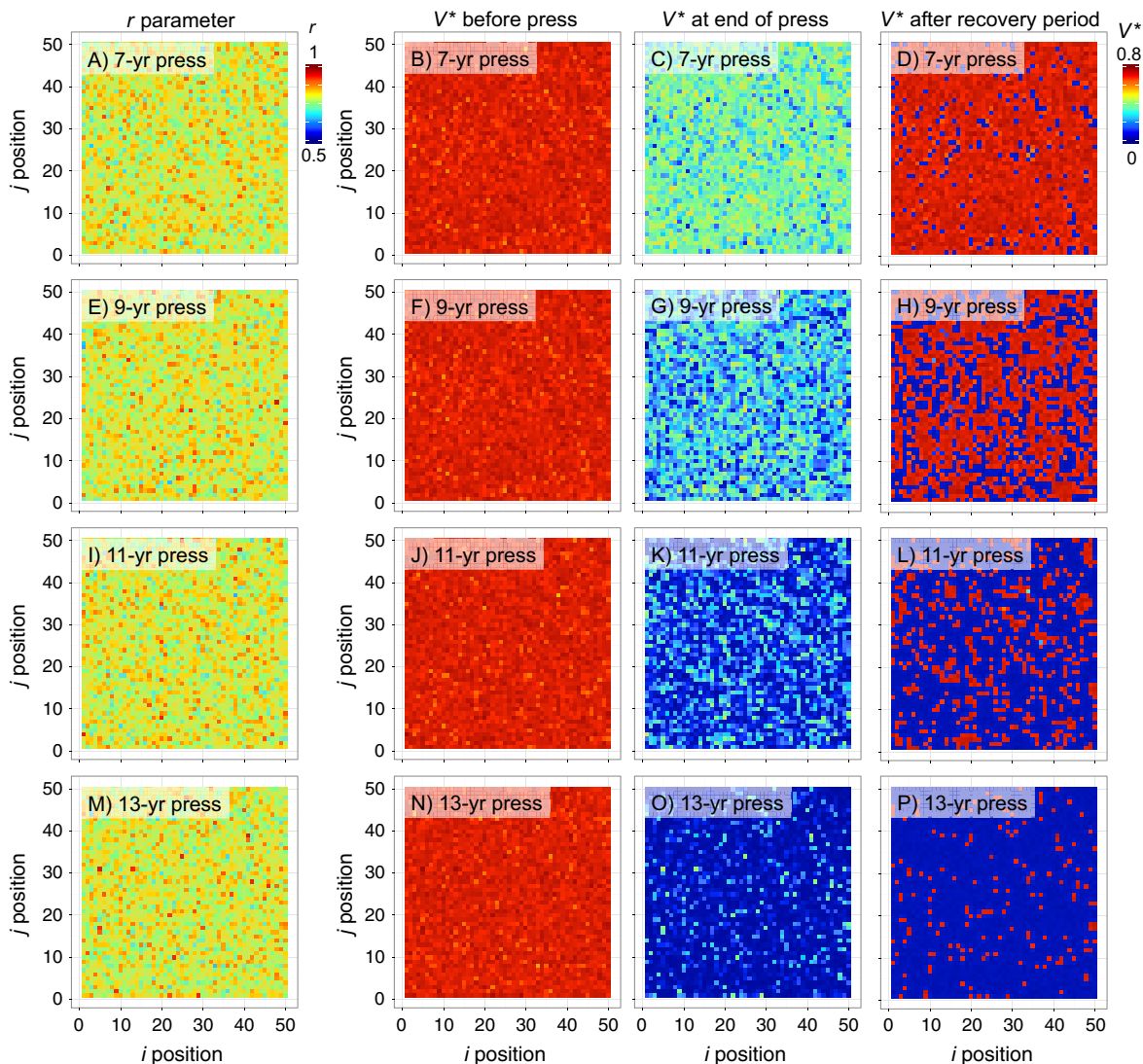
FIG. 7. Overhead views of single runs of the spatially extended model responding to a driver press with the same moderate intensity as in Fig. 6 and for varying durations of (A–D) 7, (E–H) 9, (I–L) 11, or (M–P) 13 years. The first column of panels depicts variation in the vegetation growth rate, r , with warmer colors corresponding to greater values of r (see scale to the right of panel A). The second, third, and fourth columns are overhead views of vegetation biomass, V^* , with warmer colors corresponding to greater values of V^* (see scale next to panel D). The second column depicts V^* before the press is applied, the third column is V^* at the end of the press, and the fourth column is 100 years after the press ends. In all panels, each box or “pixel” represents one patch of the system, the x -axis is dimension i and the y -axis is dimension j .
