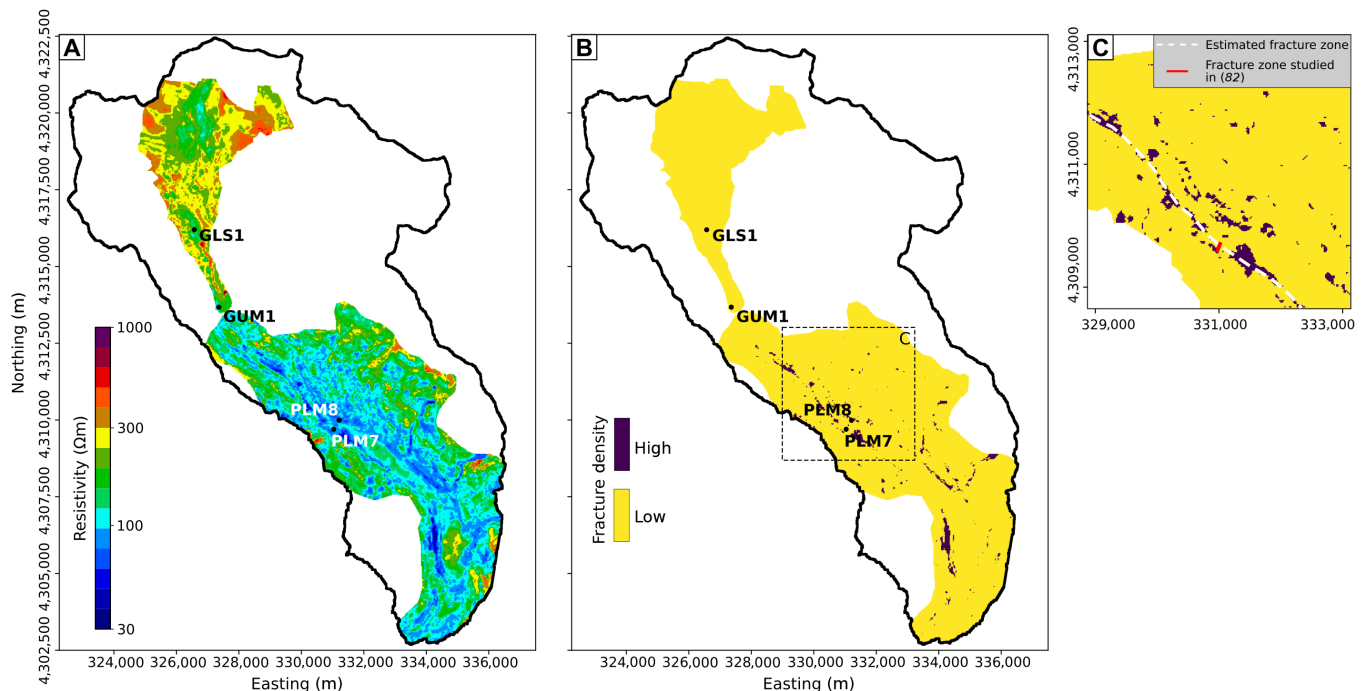
Fig. 9. Predicted shallow subsurface resistivity and fracture density. (A) Resistivity is predicted using an ERT r (73) model, using topographic elevation, slope, aspect, and vegetation type as estimators. The variation in resistivity (low resistivity in the lower watershed, high resistivity in the upper watershed) agrees with observational studies (60) showing a higher degree of metamorphism in the upper watershed. (B) Fracture density is defined on the basis of the relationship gained from the borehole data using a resistivity of 70 ohm-m. Linear features showing areas of high fracture density are postulated to correspond to fracture zones. (C) The area of the fracture zone analyzed in (83) lies along the estimated and known fracture zones.
