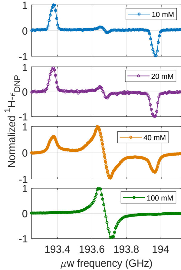
Figure 5.1: Crossover from SE to TM. Experimental ^1\text{H}\text{-}\epsilon_{\text{DNP}} vs. \nu_{\mu\text{w}} at 7 T and 20 K static condition, measured for four different Trityl-OX063 concentrations in DMSO solvent, using P_{\mu\text{w}} = 350 mW, t_{\text{buildup}} = 2 s.
