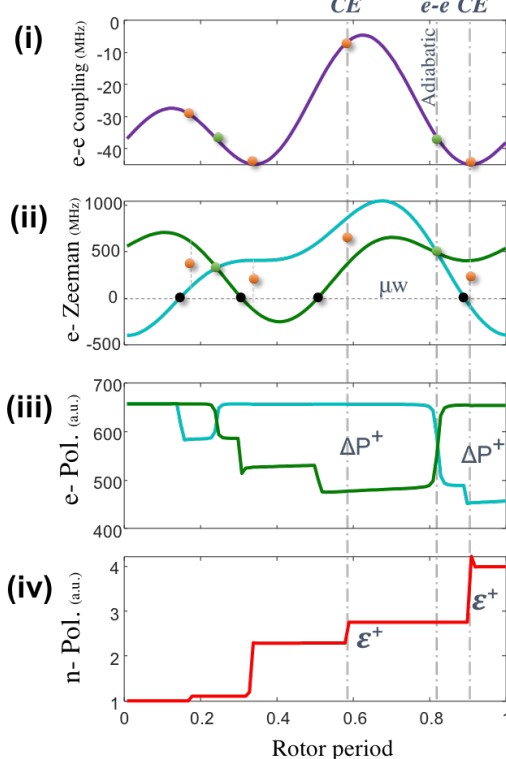
Figure 2.5: A. Landau-Zener population transition model used to rationalize spin dynamics under MAS. B. Schematic representation of essential spin transitions involved in CE DNP. C. Plot of e - e coupling (panel i ) and e -Zeeman energies in rotating frame (panel ii ), the electron and nuclear spin polarizations (panels iii and iv , respectively). The rotor events \mu w , e - e and CE are marked with black, green and orange symbols. The e - e couplings at the green e - e rotor events are large and therefore corresponding transitions are adiabatic. D. Similar to C but for a different crystallite orientation that leads to inefficient DNP. A non-adiabatic e - e event impedes the net DNP enhancement. The energies and polarizations were calculated using SpinEvolution package.
