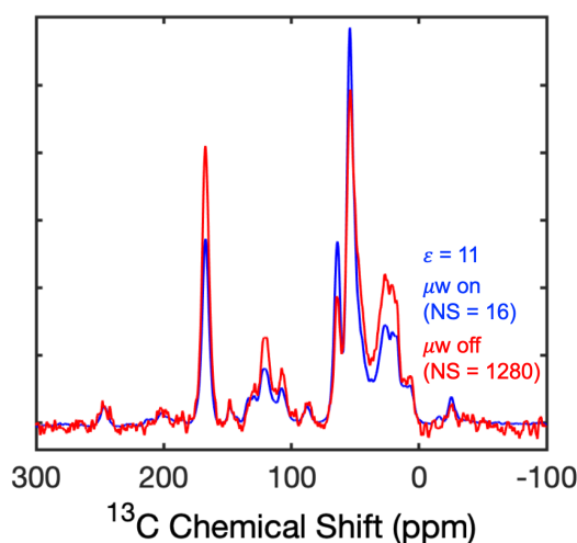
Figure 8.4: 3.5 mg [U-^{13}\text{C}] PR was prepared with POPC/POPG (80/20, mol/mol) membrane in a solvent with \text{D}_2\text{O}:\text{H}_2\text{O} = 3:1 . The ratio of PR protein to lipid is 1:50. \text{D}_8 glycerol was added to the solution and result in a solvent mixture with the ratio \text{d}_8\text{glycerol}:\text{D}_2\text{O}:\text{H}_2\text{O} = 6:3:1 . 10 mM AMUPol was dissolved for DNP experiments. Sample was packed in a 3.2 mm Bruker sapphire DNP rotor. The spectra were acquired using ^{13}\text{C} CP-MAS using a 400 MHz Bruker DNP system operating at 95 K. The buildup time used here was \text{D1} = 2 s. Blue spectra was acquired with \mu\text{w} irradiation with 16 scans. Red spectra was acquired without \mu\text{w} irradiation with 1280 scans as a comparison. DNP enhancement was calculated to be \sim 11 .
