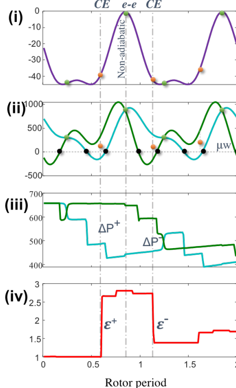
Figure 2.5: A. Landau-Zener population transition model used to rationalize spin dynamics under MAS. B. Schematic representation of essential spin transitions involved in CE DNP. C. Plot of e - e coupling (panel i ) and e -Zeeman energies in rotating frame (panel ii ), the electron and nuclear spin polarizations (panels iii and iv , respectively). The rotor events \mu w , e - e and CE are marked with black, green and orange symbols. The e - e couplings at the green e - e rotor events are large and therefore corresponding transitions are adiabatic. D. Similar to C but for a different crystallite orientation that leads to inefficient DNP. A non-adiabatic e - e event impedes the net DNP enhancement. The energies and polarizations were calculated using SpinEvolution package.
