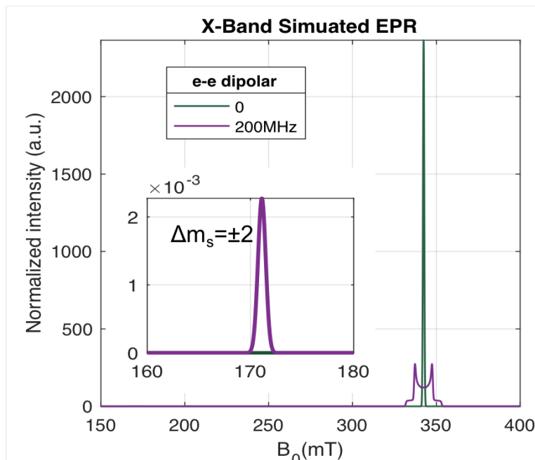
Figure 5.7: Half-field transition Easy-spin based simulated EPR spectrum for two electrons having g-anisotropy equivalent to that of Trityl, at X-band conditions. In case of strong e - e coupling, a non-negligible, \Delta m_s = \pm 2 transition is observed.
