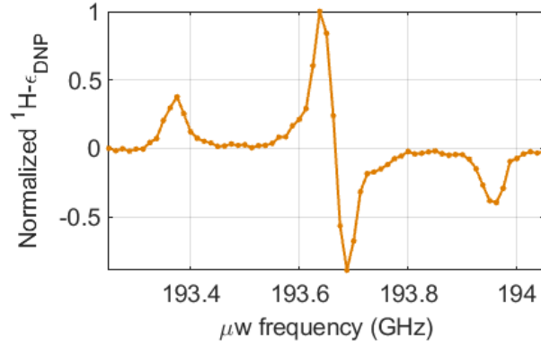
Figure 5.2: DNP frequency profile Experimental ^1\text{H}-\epsilon_{DNP} vs. \nu_{\mu w} at 7 T and 110 K, under static condition, measured for 40 mM Trityl-OX063 concentrations in DMSO solvent, using P_{\mu w} = 350 mW, t_{buildup} = 2 s.
