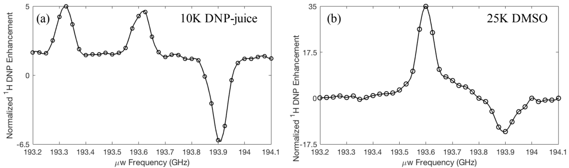
Figure 4.5: Frequency-profile of 20 mM TCP2 15 mM OX063 in (a) DNP Juice at 10 K and (b) DMSO at 25 K with 120 mW \mu w power and 60 s irradiation time.
