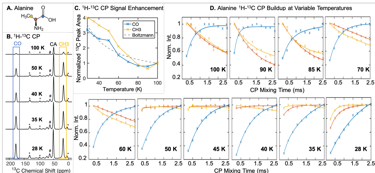
Figure 7.4: A. Chemical structure of Alanine, where the \text{CO} , \text{CA} , and \text{CH}_3 are marked with blue, red, and yellow circles, respectively. B. ^{13}\text{C} CP-MAS spectra of Ala from 100 K to 28 K. Spinning side bands are marked in * and solvent glycerol peaks are marked in #. C. ^{13}\text{C} CP-MAS \text{CO} and \text{CH}_3 peak area measured at variable temperatures. CP mixing times are optimized for \text{CO} and \text{CH}_3 separately. D. Normalized signal intensities for \text{CO} , \text{CA} , and \text{CH}_3 as a function CP mixing time at variable temperatures (from 100 K to 28 K). The solution was doped with 10 mM AMUPol.
