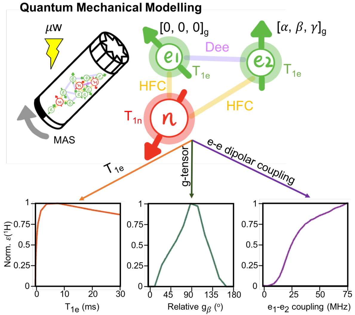
Figure 2.4: Quantum mechanical modeling of T_{1e} , relative g-tensor orientations and dipolar coupling in bis-nitroxide radicals under 25 kHz spinning in a field of 18.8 T using 0.5 MHz \mu W nutation frequency.
