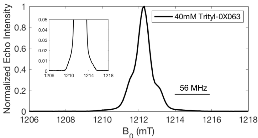
Figure 5.5: Pulse EPR Echo-detected EPR spectrum recorded for 40 mM Trityl-OX063 in \text{d}_6\text{-DMSO}/\text{D}_2\text{O}/\text{H}_2\text{O} = 76/14/10 (v/v/v) at Q-Band frequency. A 400 ns long echo delay was used to acquire the spectra. Inset shows zoomed in EPR-line at its base.
