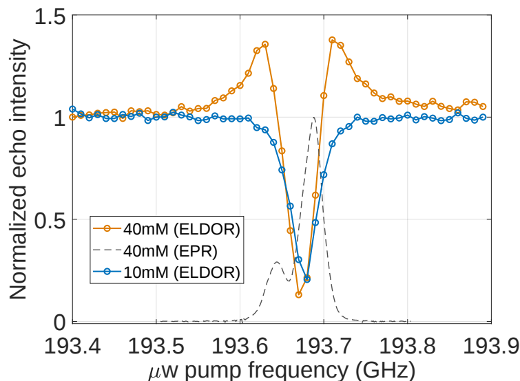
Figure 5.6: Electron hyperpolarization. Experimental ELDOR profile recorded at 20 K for 10 and 40 mM Trityl-OX063. Probe frequency was set to 193.675 GHz. A 350 mW and 50 ms long \mu w saturation pulse was used via the pump channel. Dashed line shows echo detected EPR-line of 40 mM Trityl-OX063 recorded at the same condition.
