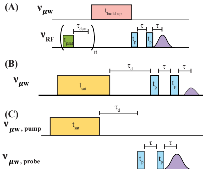
Figure 4.1: (a) Solid-echo experiment with pre-saturation pulses used for NMR experiments. Here, t_{\text{build-up}} block shows \mu w irradiation and the two short pulses ( t_p ) represent solid-echo pulses. (b) Saturation-recovery scheme to measure electron relaxation rate. The yellow block represents the electron saturation pulse and the short t_p represent echo pulses for EPR detection. The recovery time, \tau_d is changed here. (c) Two channels ELDOR pulse schematic. The \nu_{\mu w, \text{pump}} channel is to pump or saturate an electron with pulse duration ( t_{\text{sat}} ), shown in yellow block. The \nu_{\mu w, \text{probe}} channel is to probe or detect electron using solid echo pulses, shown in blue.
