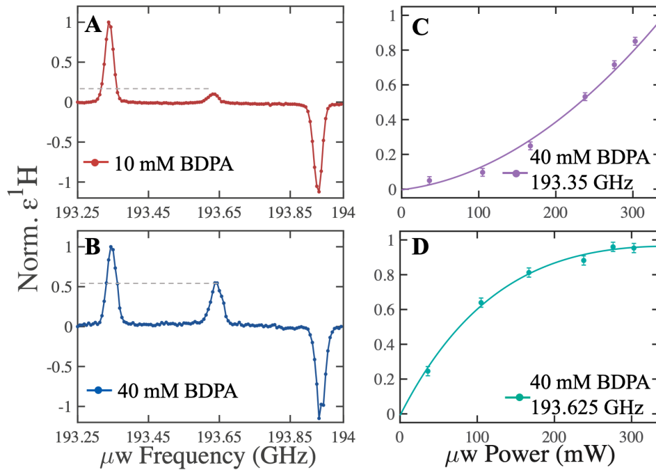
Figure 6.1: \epsilon^1\text{H} as a function of \mu\text{w} irradiation frequencies were recorded for (A) 10 mM (red) and (B) 40 mM (blue) BDPA in OTP at 20 K with \mu\text{w} irradiation power of 350 mW. The displayed \epsilon^1\text{H} was normalized by the maximum value: 5 for 10 mM BDPA and 55 for 40 mM BDPA. For 40 mM BDPA in OTP, \epsilon^1\text{H} was recorded as a function of \mu\text{w} power up to 336 mW with \mu\text{w} irradiation frequency fixed at (C) 193.35 (violet) and (D) 193.625 GHz (green). The solid lines were fitted trendlines while the dots were the experimental data with error bar (standard deviation) indicated. The build-up time was 20 s for ^1\text{H} DNP measurements.
