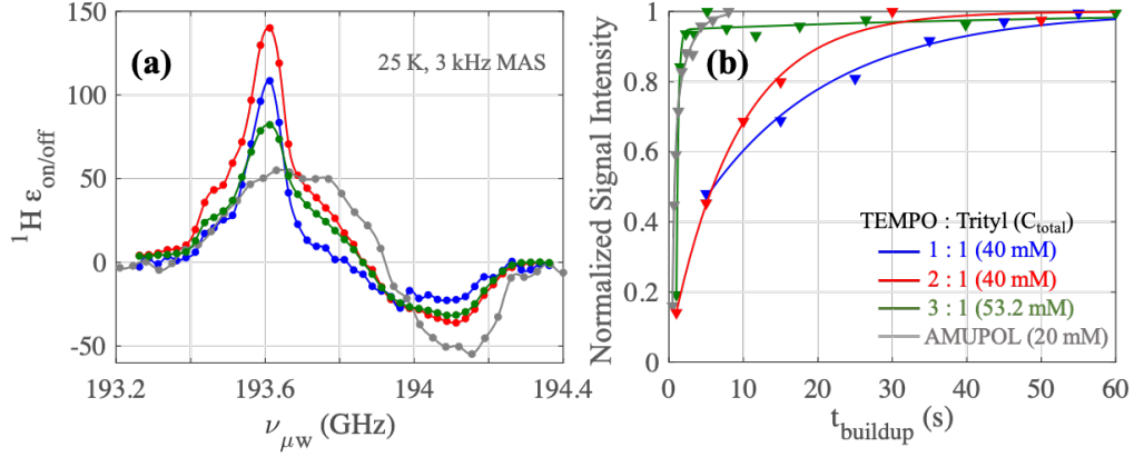
Figure 3.4: (a) Experimental ^1\text{H}\epsilon vs. \nu_{\mu\text{w}} at 3 kHz MAS, 25 K for TEMPO:Trityl = 1:1 ( C_{\text{total}} = 40 mM, blue), 2:1 ( C_{\text{total}} = 40 mM, red), and 3:1 ( C_{\text{total}} = 53.2 mM, green), and C_{\text{total}} = 20 mM AMUPol in DNP Juice, measured using 2\text{-}^{13}\text{C} glycine through ^1\text{H}\text{-}^{13}\text{C} CP experiment. P_{\mu\text{w}} = 350 mW and t_{\text{buildup}} = 60 s. (b) DNP buildup at optimum \nu_{\mu\text{w}} .
