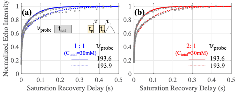
Figure 3.1: Saturation recovery T_{1e} measurement at 4 K for two different radical-mixtures: (a) TEMPO:Trityl = 1:1 ( C_{total} = 30 mM, blue), (b) 2:1 ( C_{total} = 30 mM, red). The grey crosses are normalized electron echo intensities as a function of \tau_D , and the solid and dotted lines are the two-component fitting curve for \nu_{probe} set at Trityl (193.6 GHz) and TEMPO (193.9 GHz) center frequencies, respectively.
