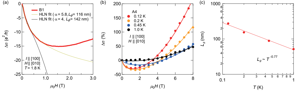
FIG. 3. (a) Magnetoconductance \Delta\sigma = \sigma(H) - \sigma(0) at 1.8 K for the B1 microstructure. The solid thin yellow and black lines show fits to the Hikami-Larkin-Nagaoka (HLN) model (Eq.(3)). In the latter case, \alpha is fixed to 4. (b) Magnetoconductance of the A4 single crystal for different temperatures. The solid lines are the fits to the HLN model. (c) Temperature dependence of the dephasing length L_\phi in the A4 single crystal. The line is the fit to T^{-\gamma} .
