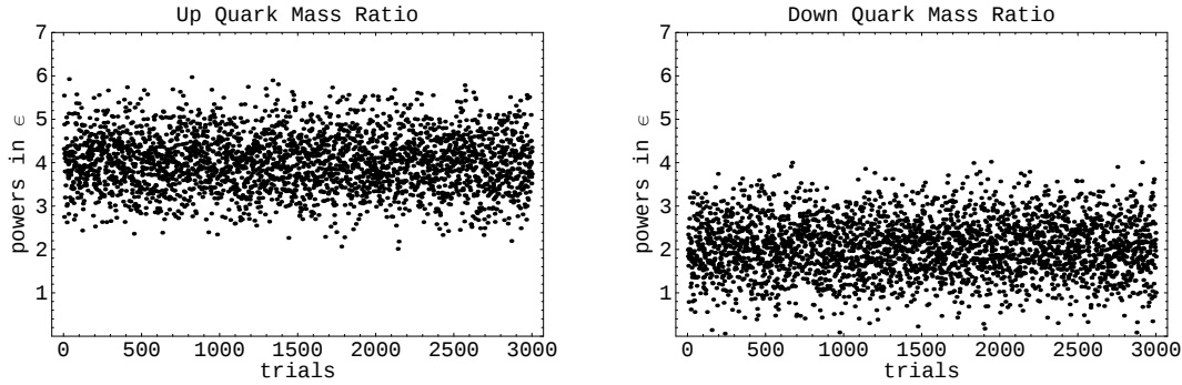
Figure 3: The powers in \epsilon of the ratios \frac{m_u}{m_c} and \frac{m_d}{m_s} .
