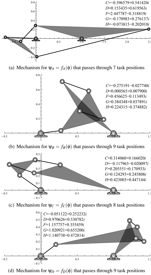
Fig. 7. The four linkage solutions which were selected to mechanize the magpie wing trajectory. All linkages possess a fully rotatable input crank
