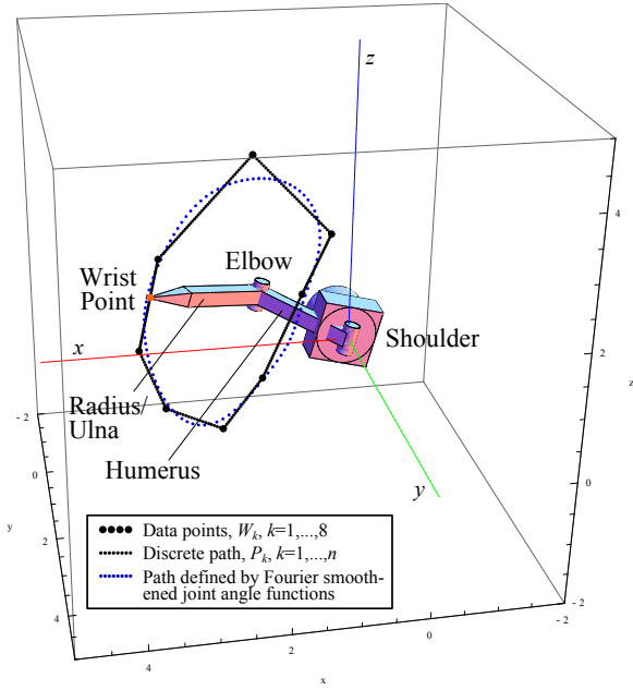
Fig. 3. The sequence of points \mathbf{P}_k, k = 1, \dots, n is shown in black. By fitting Fourier series to the discrete joint angle functions for \psi_A, \psi_B, \psi_C , a new smoother trajectory is generated shown in blue
