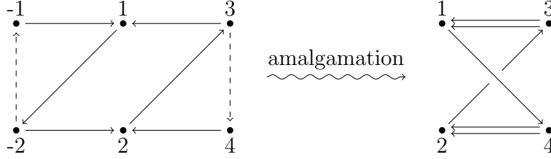
Figure 5.1: The quivers of \Sigma_i and \Sigma_C when C is of type A_2 . The dashed arrows correspond to entries of B_i equal to \pm\frac{1}{2} ; since they connect frozen vertices they do not affect the structure of cluster transformations, but record the Poisson brackets among frozen variables. The amalgamation itself “glues together” some of the frozen variables: -1 to 3 and -2 to 4 .
