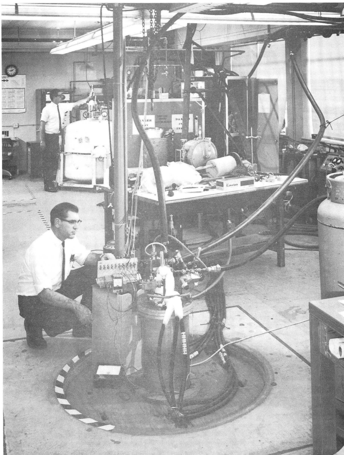
Fig. 3. A one-meter long dipole cryostat (foreground) being run from the LRL refrigerator (background) through a 50-foot long coaxial transfer line (black hose entering the cryostat from the top of the picture).
