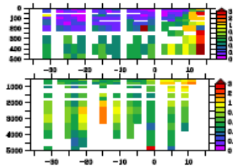
BLING, GA-03
