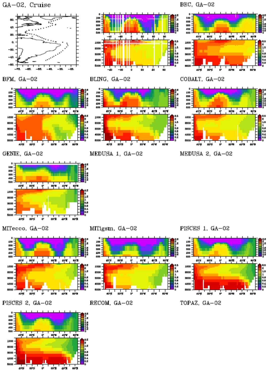
Figure 10. \text{PO}_4 concentrations ( \mu\text{M} ) from the GA-02 cruise [Rijkenberg et al. , 2014] and extracted from the FeMIP models ( \text{PO}_4 not provided for MEDUSA-1, MEDUSA-2, RECOM and TOPAZ).
