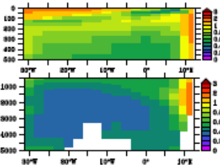
TOPAZ, GA-03
