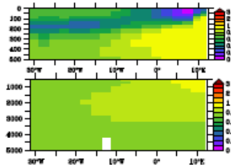
RECOM, GA-03
