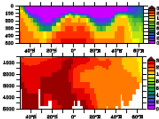
BFM, GA-02
