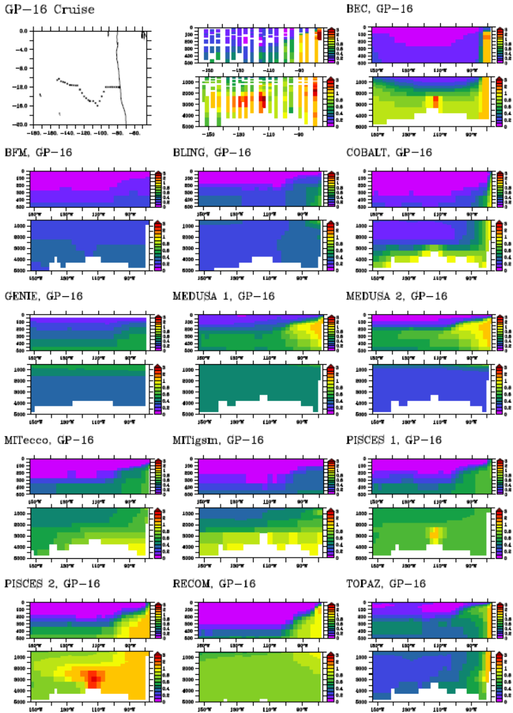
Figure 7. DFe concentrations (nM) from the GP-16 cruise [Resing et al. , 2015] and extracted from the FeMIP models.
