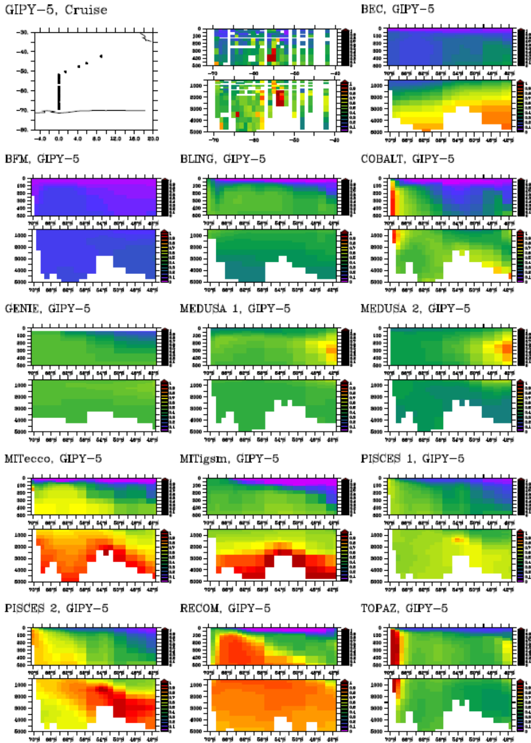
Figure 8. DFe concentrations (nM) from the GIPY-4 and 5 cruises [Chever et al. , 2010; Klunder et al. , 2011] and extracted from the FeMIP models
