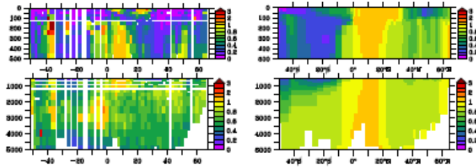
BLING, GA-02
