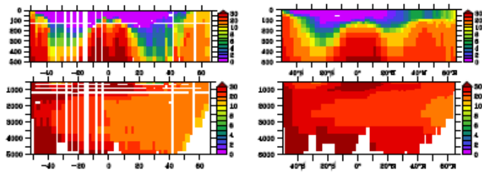
BLING, GA-02
