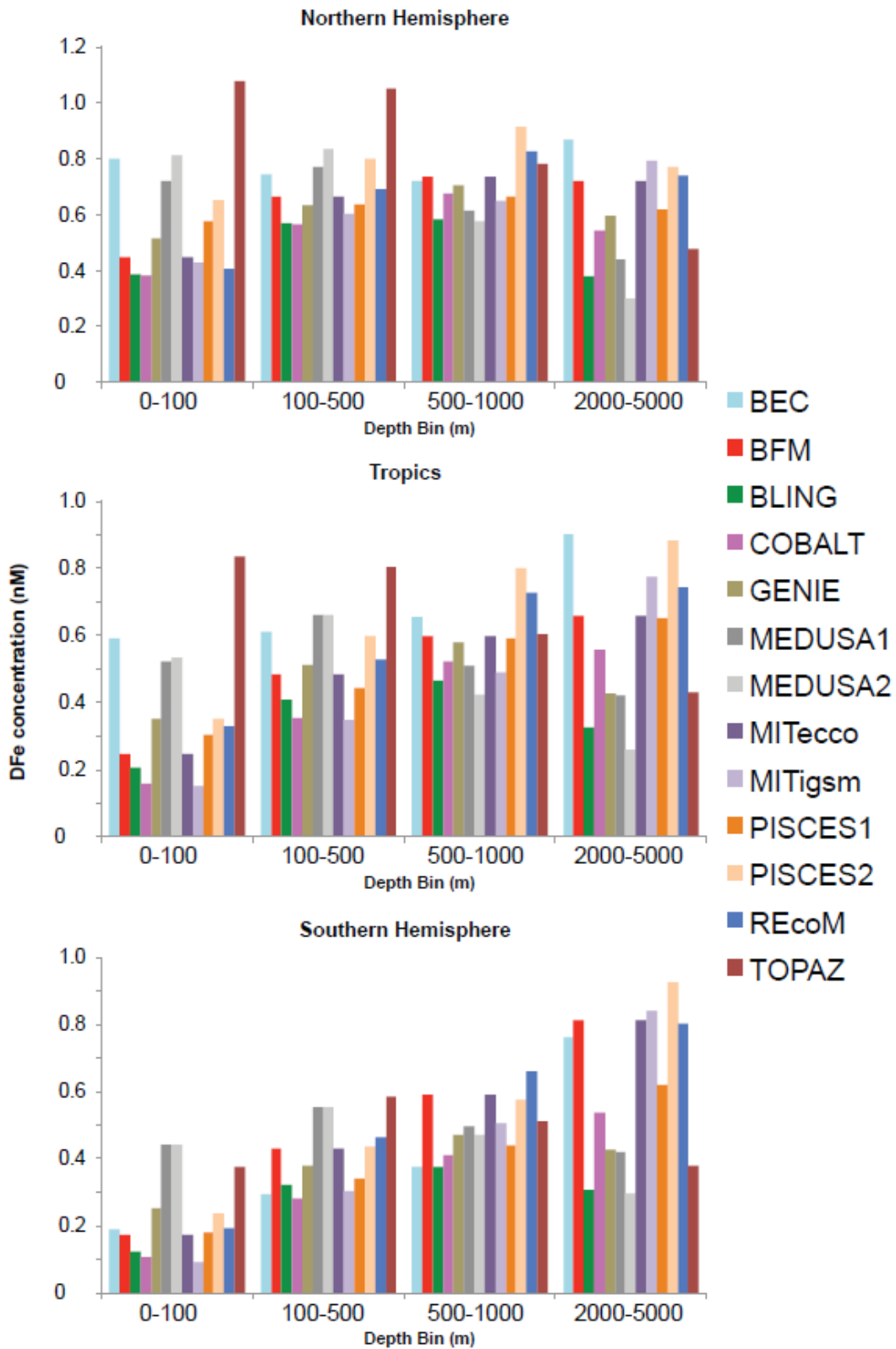
Figure 1. Histograms of the average DFe concentration (nM) simulated by the FeMIP models across four different depth bins for three regions. The Northern Hemisphere is 30°N-90°N, Tropics are 30°S-30°N and the Southern Hemisphere is 30°S-90°S.
