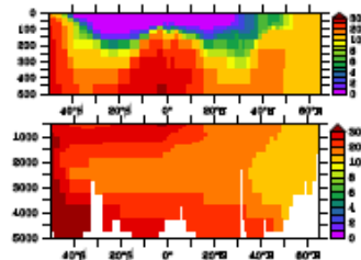
MEDUSA 2, GA-02
