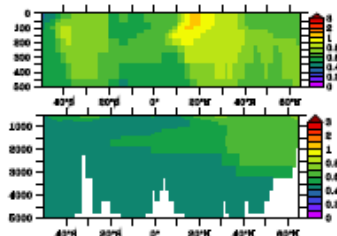
MITigsm, GA-02
