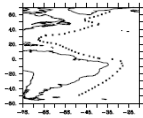
BFM, GA-02
