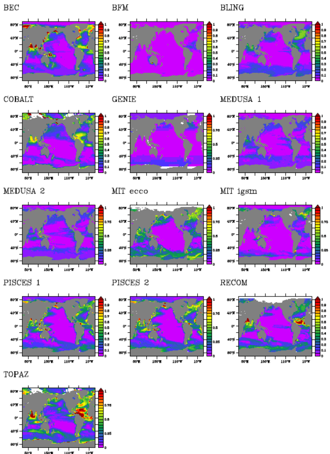
Figure 3. Annual maximum minus annual minimum DFe concentrations (nM) averaged over the upper 50m from the FeMIP models.
