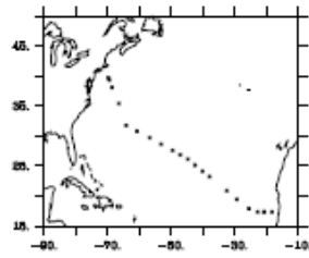
BFM, GA-03
