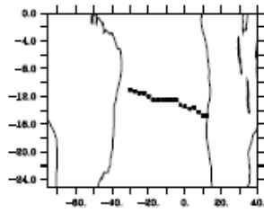
BFM, GA-03
