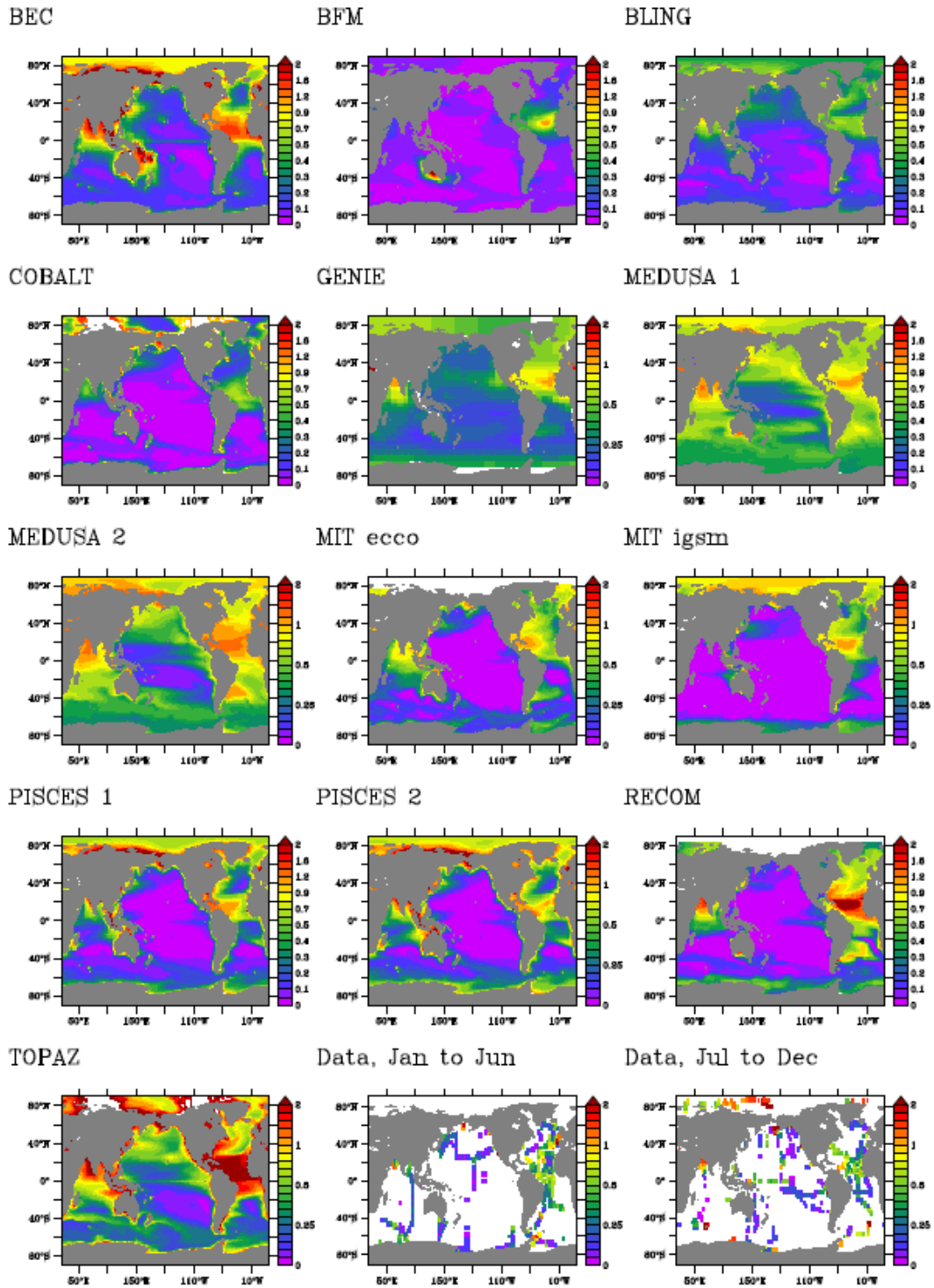
Figure 2. Annual mean DFe concentrations (nM) averaged over the upper 50m from the FeMIP models. Data averaged over the period January to June and July to December is taken from the expanded Tagliabue et al. [2012] dataset and has been averaged over 5° bins in latitude and longitude to improve visibility.
