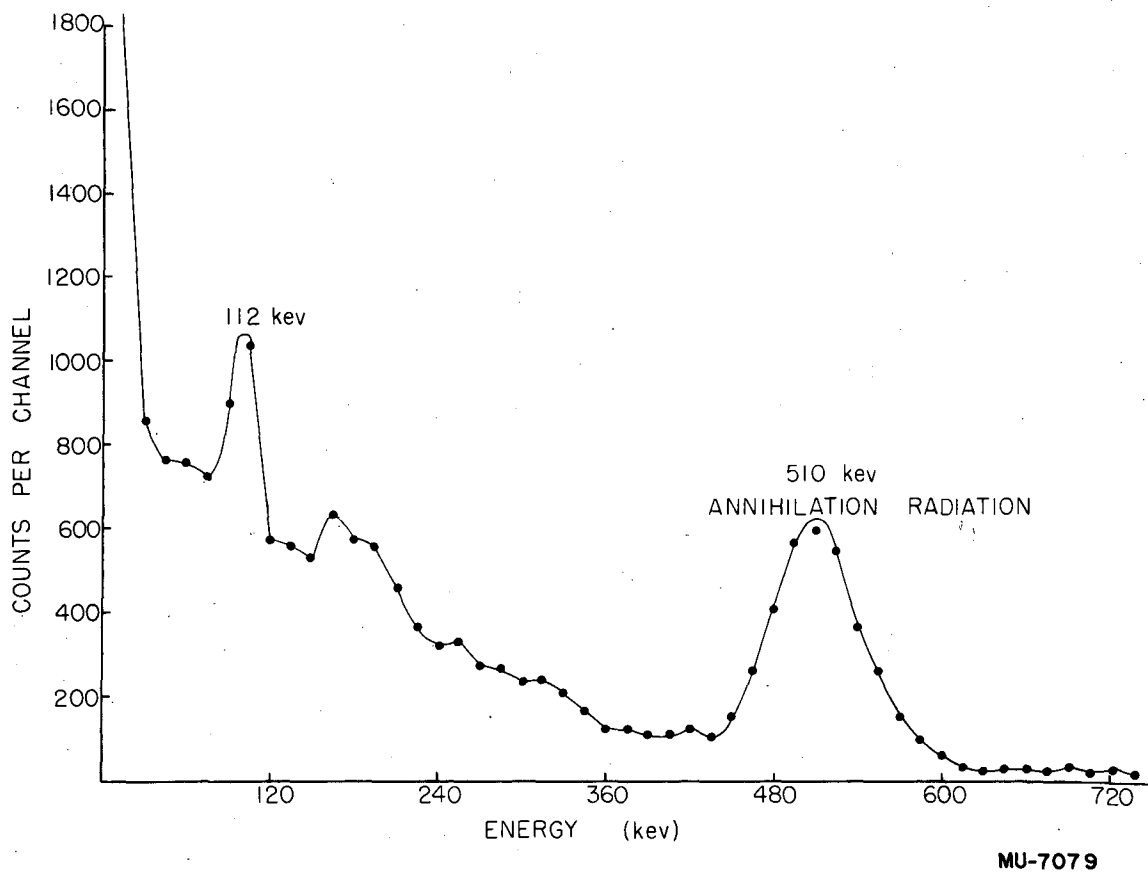
Fig. 13. Gamma spectrum of mass-separated Cs^{125} in 0-600 keV region.
