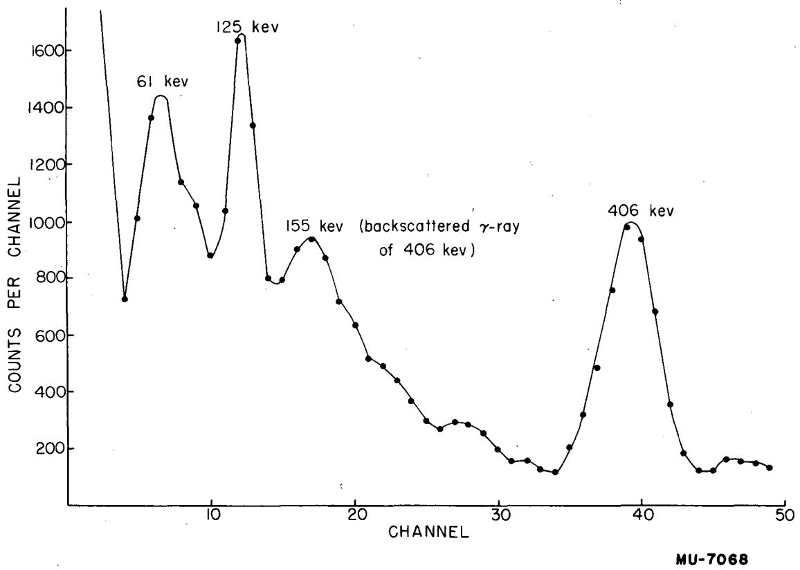
Fig. 2. Gamma spectrum of mass-separated \text{Cs}^{127} determined in scintillation spectrometer.
