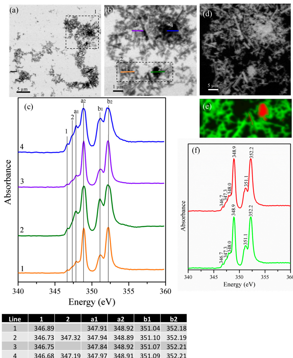
Figure 7. (a) Image taken at the calcium L_{II,III} edge of the mix of the cubic C_3A and the gypsum sample at a ratio of 1.9; (b) magnification of area 1 in (a); (c) NEXAFS spectra of the line scans indicated in (b); (d) image maps of calcium in the same area as in Figure 6b, where the brighter areas are related to higher concentrations of calcium; (e) image stack (red and green areas correspond to ettringite crystals); (f) RGB composite map of region 2 in Figure 7b; and (g) NEXAFS spectra of the red and green regions observed in (e).
