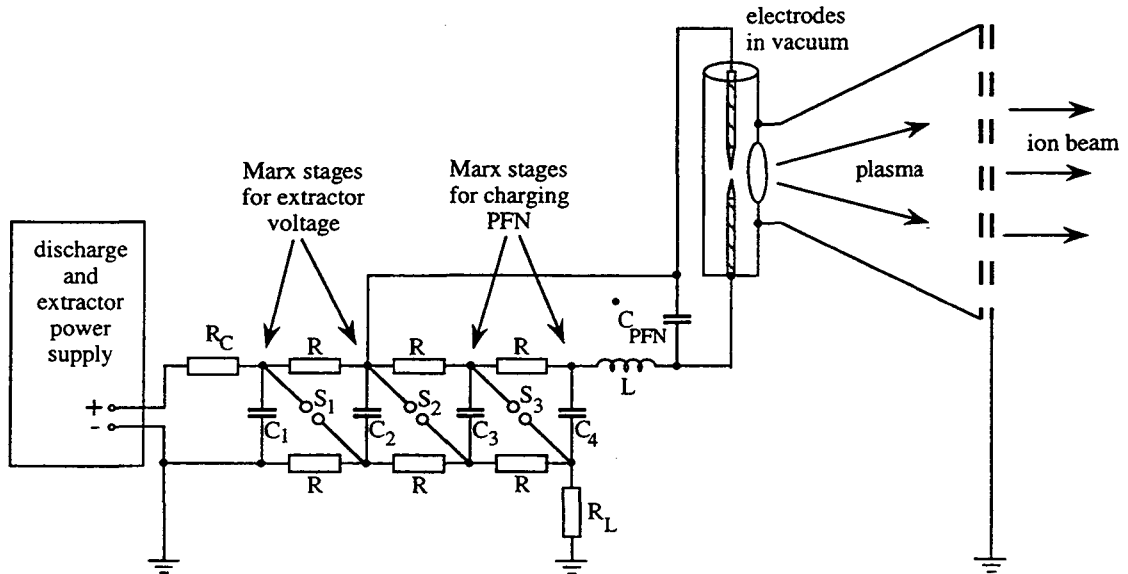
Fig. 2 Principal electrical scheme of "Magis". The pulse forming network is symbolically represented by a lumped capacitor, C_{PFN} ; L - inductive resistor (coil); the other notation is as in Fig. 1.
