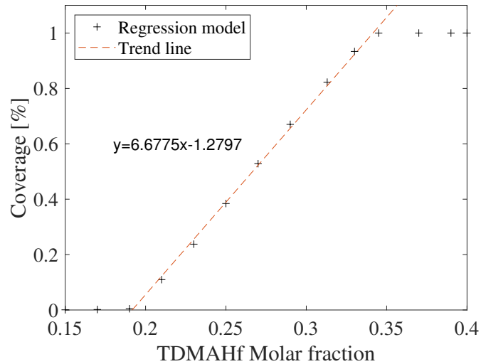
Figure 5.4: The input-output relationship between the final film coverage and the precursor molar fraction derived from linear regression used in both EWMA and PCC-based R2R controller. The y-axis is the final coverage and the x-axis is the inlet TDMAHf molar fraction.
