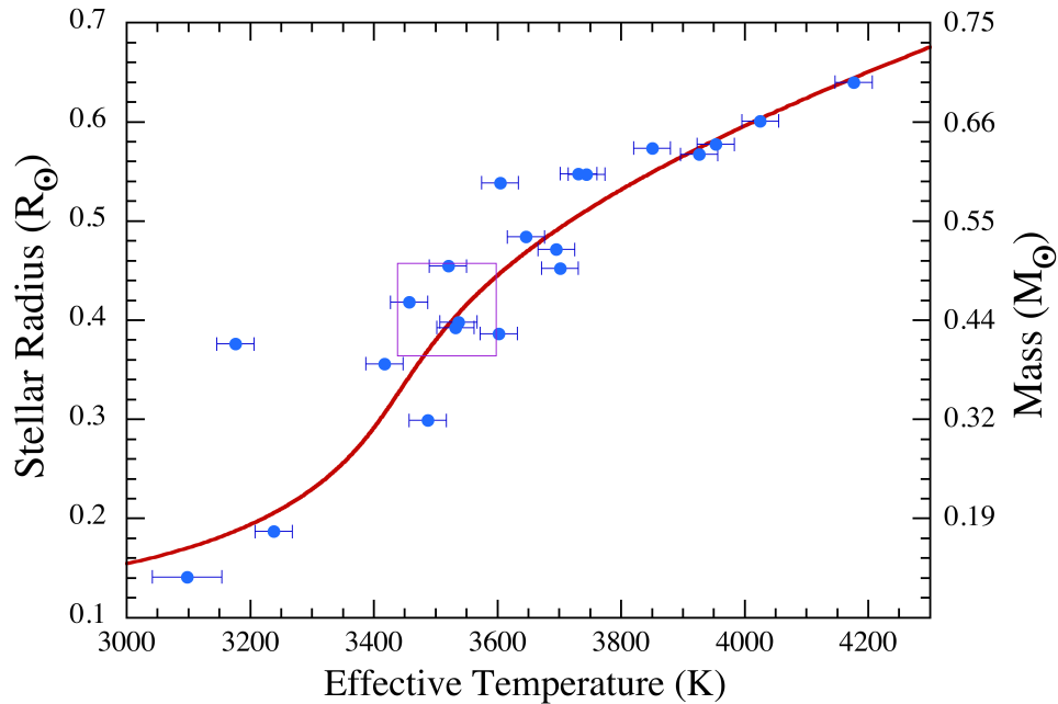
FIG. 18.— Model stellar radius vs. effective temperature relation on the lower main sequence for solar metallicity stars. The red curve is a parametric expression plotted from Eqns. (A1) and (A2). The blue circles with error bars are taken from the work of Demory et al. (2009), Boyajian et al. (2012), and Newton et al. (2015). The purple box is the region within which most of our results are derived. The masses listed on the right-hand axis are parametrically inferred from Eqns. (A1) and (A2) and are not measured.
