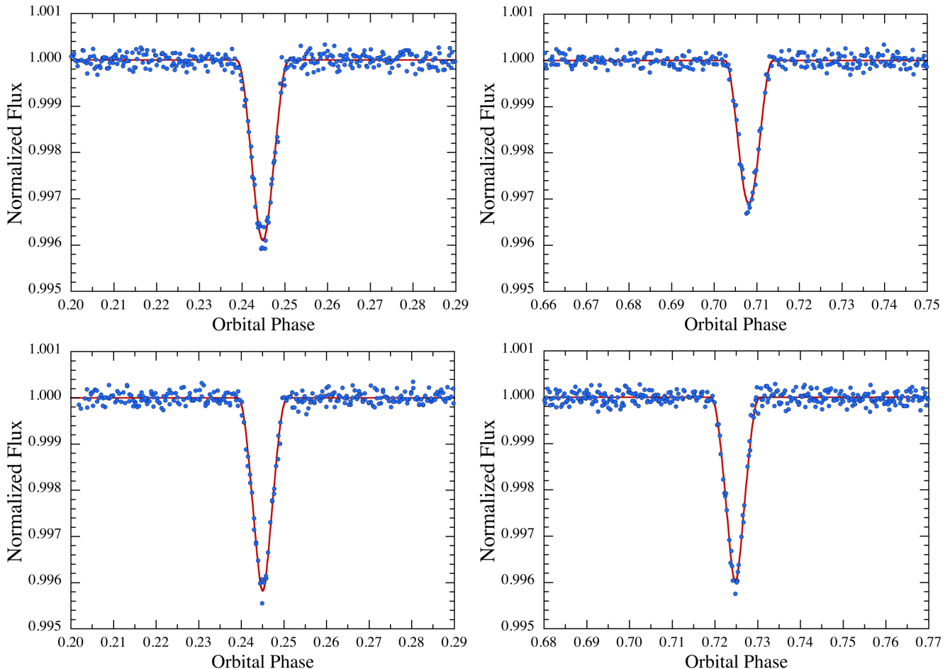
FIG. 9.— K2 eclipse profiles for the primary and secondary eclipses in both the A binary (top panels; P_{\text{orb}} = 13.27 d) and the B binary (bottom panels; P_{\text{orb}} = 14.41 d). Each profile contains data from \sim 5 eclipses. Orbital phase zero is arbitrary, but correctly gives the relative phases of the primary and secondary. The absolute times of the primary eclipse (defined as those in the left panels) are given in Table 4. The red curve is a best fitting model which includes 6 independent parameters for each binary system (see Sect. 6).
