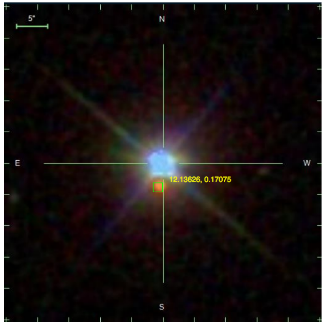
FIG. 2.— SDSS image showing the region near EPIC 220204960. We have designated the brighter bluish colored image to the north as ‘B-N’ while the fainter reddish image some 3'' to the south is designated as ‘R-S’. The ‘R-S’ image hosts both binaries in a bound quadruple system.
