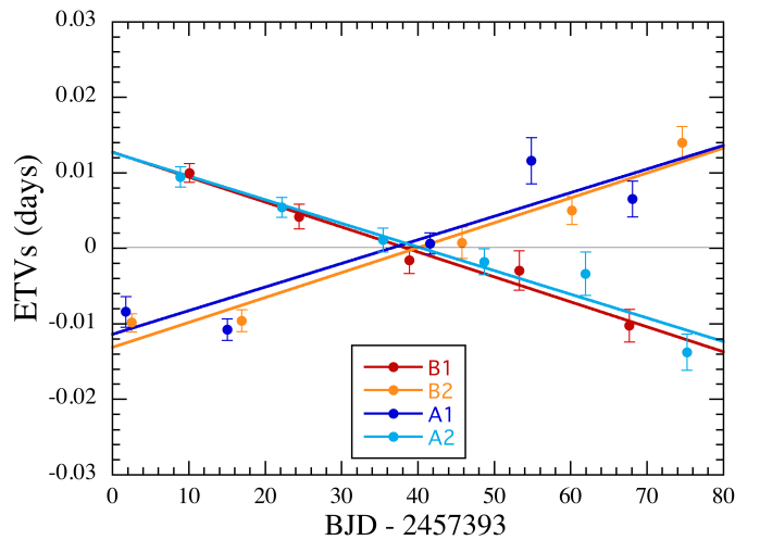
FIG. 8.— Eclipse timing variations in the arrival times of all four eclipses in the two binaries that comprise EPIC 220204960. In each case the mean orbital period for each binary has been used to produce the ETV curves. Note the strong divergence of the ETV curves for the primary and secondary eclipses of both the A and B binaries. See Table 4 for a summary of periods and ETVs.
