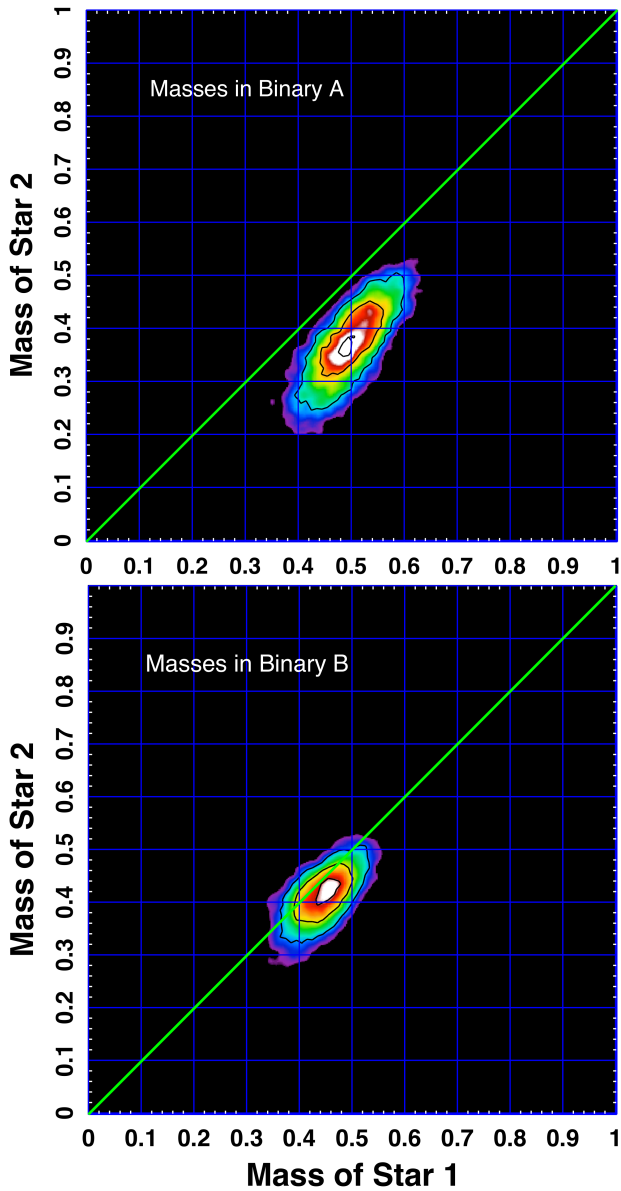
FIG. 10.— Correlation plot between M_1 and M_2 for both binaries taken from the output of the MCMC fit to the eclipses.
