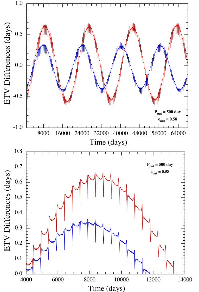
FIG. 12.— Simulated ETV curves for an illustrative outer orbit of binary A around binary B with P_{\text{orb}} = 500 d and e_{\text{out}} = 0.58 . The red and blue curves are the ETV differences between the primary and secondary eclipses for the A and B binaries, respectively (with the mean difference P_{\text{bin}}/2 subtracted). We plot the ETV differences because that is what the relatively short K2 observations are able to measure.
