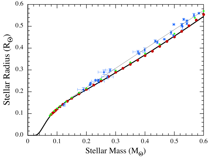
FIG. 16.— Model stellar radius vs. mass relation on the lower main sequence for solar metallicity stars. The red circles are models that we generated for this work (see text). The light green circles are taken from the Baraffe et al. (1998) results. The solid black curve is the log-polynomial fit (Eqn. A1) to our model points (in red). Blue circles with error bars are well-measured systems (see, e.g., Cakirli et al. 2010; Kraus et al. 2011; Carter et al. 2011b; Dittmann et al. 2016, and references therein). The grey straight line marks the trend of the data points away from the models.
