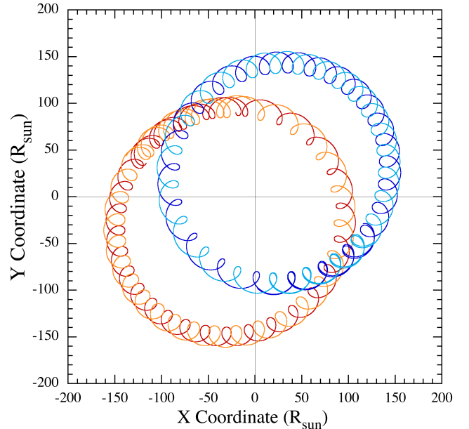
FIG. 14.— Orbital motion of the EPIC 220204960 quadruple system for an assumed illustrative outer orbital period of 500 days and eccentricity of 0.3. The orbital tracks of all four stars are shown in different colors.
