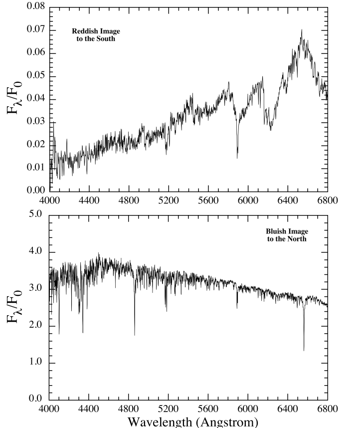
FIG. 3.— MDM 2.4-m spectra of the ‘R-S’ image (top panel) and ‘B-N’ star (bottom panel). The spectra have been corrected for the throughput efficiency as a function of wavelength. The reference flux density, F_0 , is 10^{-14} \text{ergs cm}^{-2} \text{s}^{-1} \text{Å}^{-1} . The ratio of detected flux in the two spectra is \sim 100 . This implies a ratio of \sim 60 in the Kepler bandpass after correcting for the red flux between 6800 \text{Å} and 8500 \text{Å} that is not included in the spectrum.
