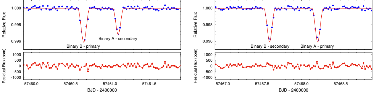
FIG. 11.— Characteristic portions of the K2 lightcurve together with the synthetic simultaneous solution lightcurve (upper panel), and the residual curve (below). Note that the two eclipses shown in each panel are for two different binaries.
