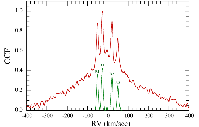
FIG. 6.— Cross correlation (red curve) between the HIRES spectrum and the template from a reference M star. After subtracting off a pedestal of broader features, the green curve shows the four peaks more clearly that correspond to the four M stars in the quadruple star system. The inferred radial velocities, which range from -50 \text{ km s}^{-1} to +50 \text{ km s}^{-1} , are about as expected near quadrature for the two binaries.
