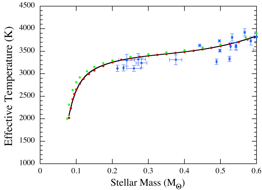
FIG. 17.— Model stellar effective temperature vs. mass relation on the lower main sequence for solar metallicity stars. The symbols and color coding are the same as in Fig. 16. The solid black curve is the fit of Eqn. (A2) to our model points (in red).
