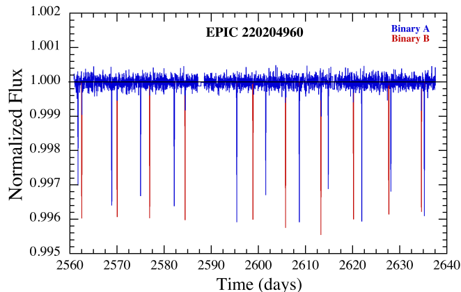
FIG. 1.— K2 flux data for EPIC 220204960. The eclipses of the 13.27-day ‘A’ binary are colored in blue, while those of the 14.41-day ‘B’ binary are in red. All four eclipses are of comparably shallow depth. We note that this lightcurve contains the light of the bright northerly blue stellar image designated ‘B-N’ (see Fig. 2). At \sim 3'' separation from the ‘A’ and ‘B’ binaries, the fluxes are not separable with K2.
