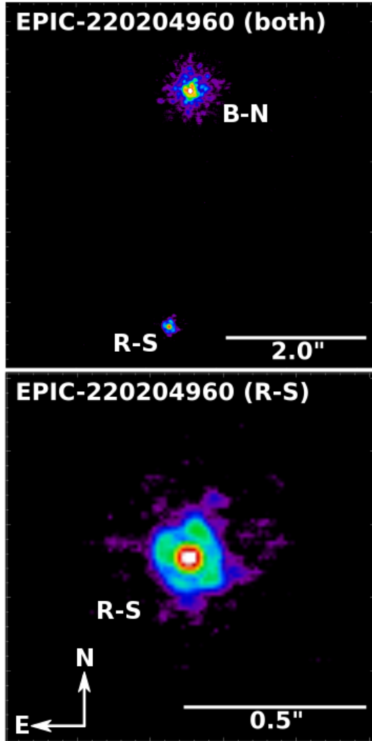
FIG. 5.— Top panel: Keck-AO image in K_s -band of EPIC 220204960, including the brighter blue image to the north, ‘B-N’, and the fainter red image 3''.4 to the south, ‘R-S’. A zoom-in on the ‘R-S’ image which hosts the quadruple system, is shown in the bottom panel. If the two binaries were separated by 0''.1 or more, the core of the image would be cleanly split into two objects. A separation of even 0''.05 would produce a noticeably elongated central core, which is not seen.
