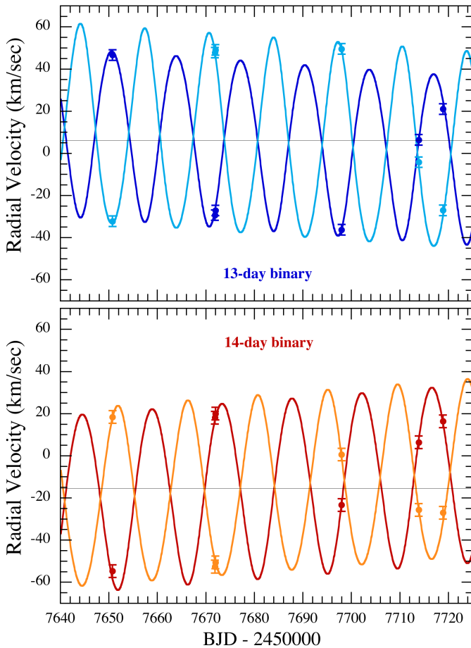
FIG. 7.— Radial velocity measurements from two IGRINS and four HIRES spectra. The second of the IGRINS spectra has nearly the same epoch as the HIRES spectrum. Top panel is for the 13-d A binary and bottom panel for the 14-d B binary. The solid curves are the best fits with only the K velocity of each star, the \gamma velocity (black horizontal line), and \dot{\gamma} as free parameters for each binary, while \omega , \tau , and e are taken from Table 6.
