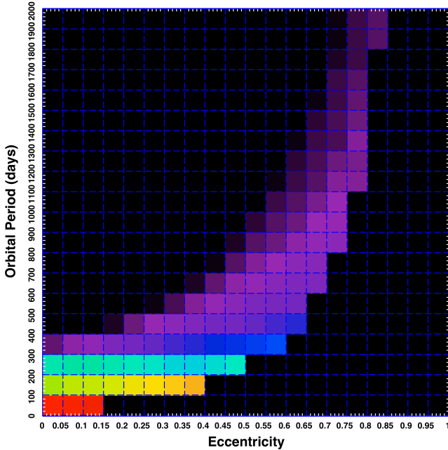
FIG. 13.— Exploration of the P_{\text{out}} - e_{\text{out}} plane to determine the importance of dynamically driven apsidal motion in the EPIC 220204960 quadruple system. The colors indicate the fraction of time during P_{\text{out}} when the induced ETVs over the course of 80 days match or exceed those observed during the K2 observations. Red, orange, cyan, blue, purple, and dark purple represent 90%, 80%, 40%, 25%, 10%, and 1%, respectively.
