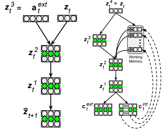
Figure 3: (Left) The CogNGen dynamics model. (Right) The CogNGen motor-action model. Arrows transform data across synapses. Gray circles represent stateful neurons and green diamonds represent error neurons. In the motor model, the internal control portion produces signals \mathbf{c}_t^{int} that manipulate working memory and the external control portion transmits signals \mathbf{c}_t^{ext} that affect the environment. Note that both internal and external control share the same working memory.
