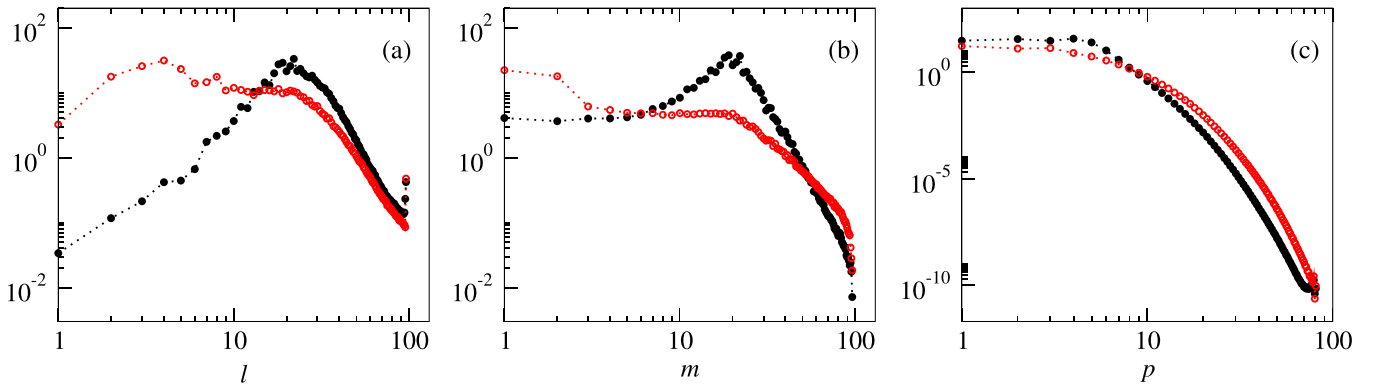
Figure 1. Time-averaged power spectra of kinetic (full circles) and magnetic (empty circles) energy as a function of (a) the harmonic degree l , (b) the harmonic order m , and (c) the Chebyshev polynomial degree p in the case \eta = 0.65 , R = 6 \times 10^6 , Pr = 1 , Pm = 2 , \tau = 2000 , n = 2 , N_p = 3 .
