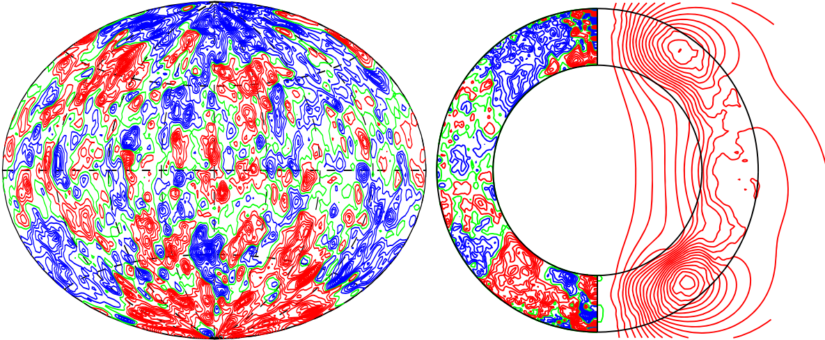
Figure 7. Magnetic field components of the same case as in the right column of Figure 6. The left plot shows contours of B_r at r = 1.13 + r_i , and the right plot shows contours B_p and meridional field lines.
