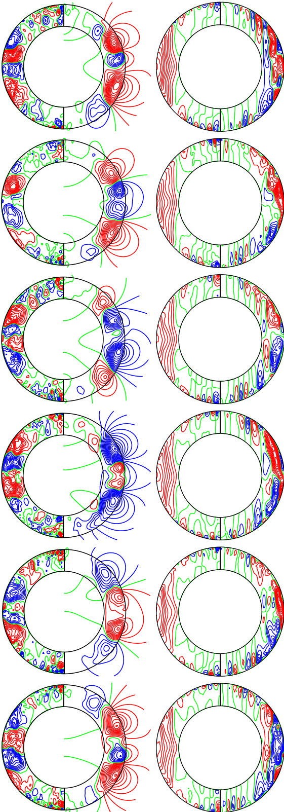
Figure 9. One period of dipolar oscillations in the case \eta = 0.65 , \text{Pr} = 1 , \tau = 2 \times 10^3 , R = 2.5 \times 10^6 , \text{Pm} = 4 , n = 2 , N_p = 3 with the no-slip condition on the inner boundary. Time between plots is \Delta t = 0.09 starting at t_0 = 96.8174 in the time series shown in Figure 10. The first row shows contours \vec{B}_p to the left and meridional field lines to the right. The second row shows contours \vec{B}_\phi to the left and the streamlines r \sin \theta (\partial_\theta \vec{v}) to the right, all in the meridional plane.
