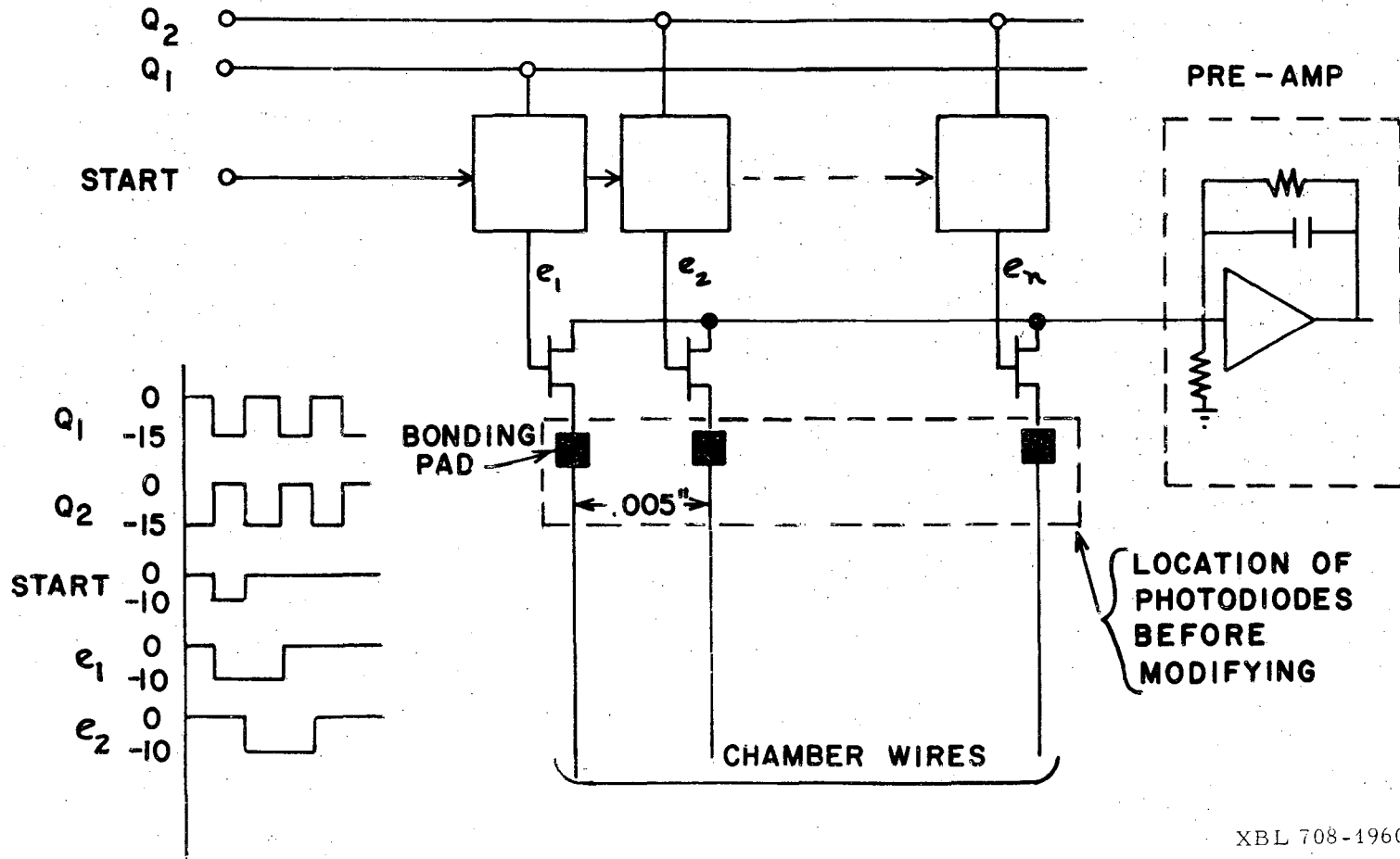
Fig. 19. Self-scanned switching array circuit diagram.
