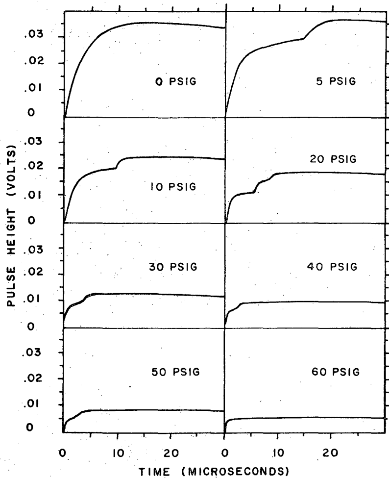
Fig. 13. Pulse shape as a function of pressure for the shorter type of pulse seen in liquid argon on etched tungsten tips.
