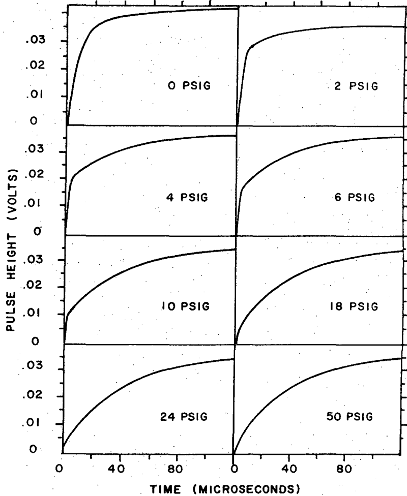
Fig. 14. Pulse shape as a function of pressure for the longer type of pulse seen in liquid argon on etched tungsten tips.
