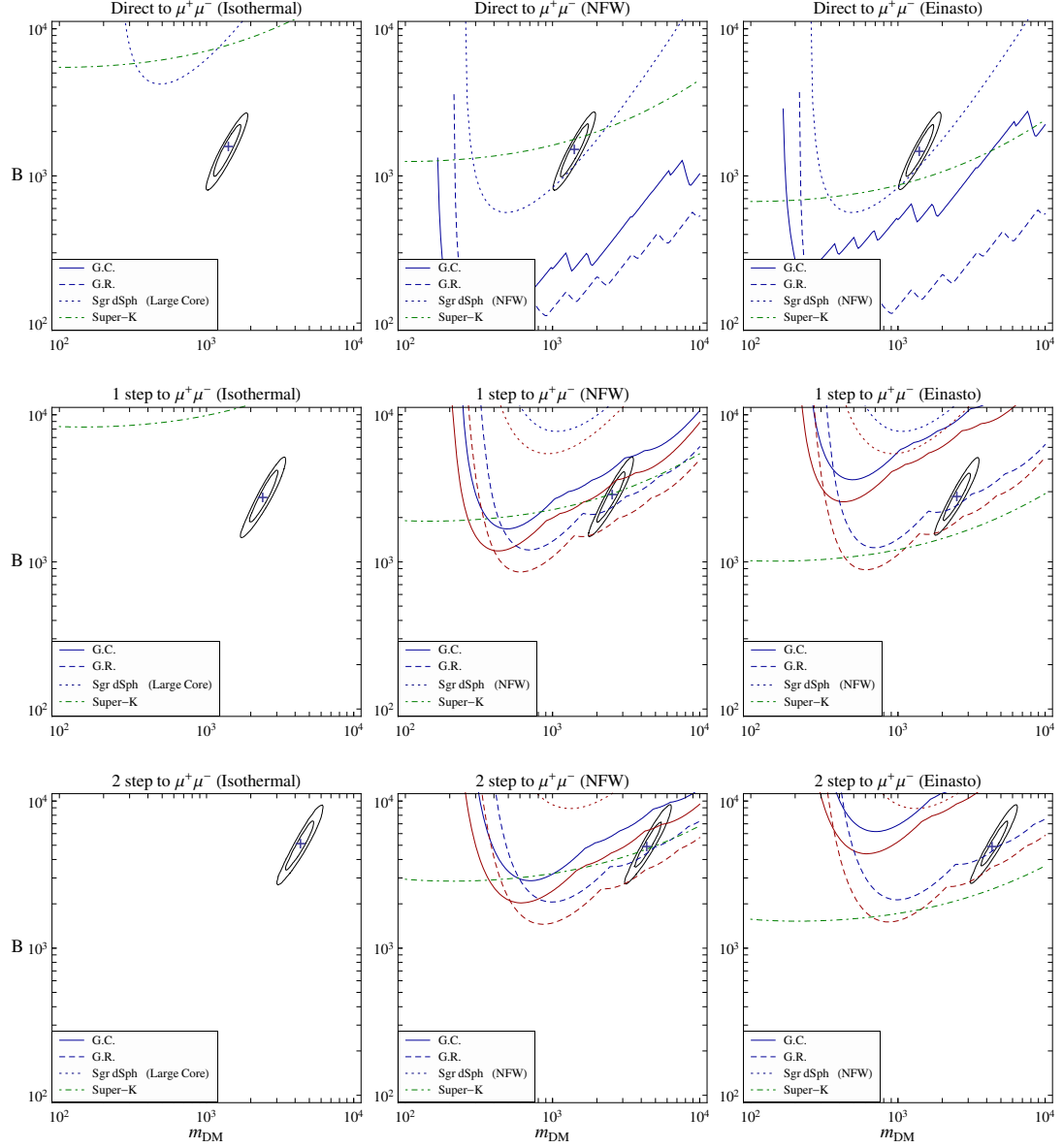
Figure 2.7: The same as Figure 2.6 but for muon final states. Also included are constraints from neutrino observations (dot-dashed) assuming B_{\nu, \text{astro}} = B_{e, \text{astro}} . For cascade annihilations, the upper (blue) and lower (red) curves now correspond to m_1 = 600 MeV and 1 GeV, respectively.
