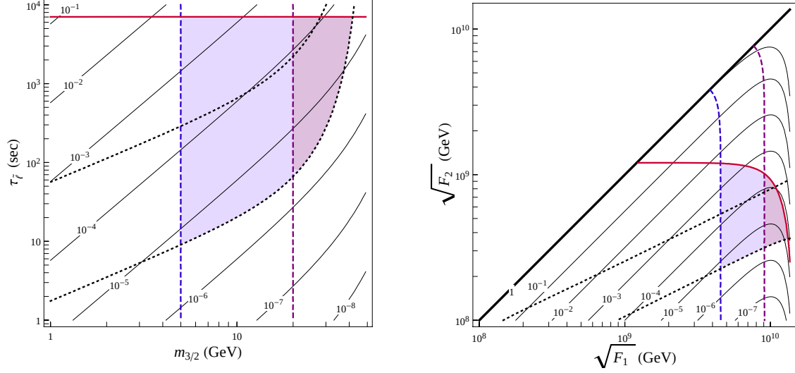
Figure 4.2: Contours of the branching ratio \Gamma_{\tilde{\ell} \rightarrow \ell \tilde{G}}/\Gamma_{\tilde{\ell} \rightarrow \ell \zeta} (labeled, solid black) together with constraints from cosmology and collider physics for m_{\tilde{\ell}} = 100 GeV, shown in the m_{3/2} - \tau_{\tilde{\ell}} plane (left) and in the \sqrt{F_1} - \sqrt{F_2} plane (right). The BBN bound excludes the parameter regions above the solid red lines, while goldstino overproduction from SSM sfermion decays excludes the regions below the dotted lines (the two dotted lines in each plot correspond to r \equiv m_{\tilde{Q}}/m_{\tilde{L}} = 3 (lower) and 10 (upper); see Sec. 4.5.1). Demanding that the gravitino is heavy enough to be measured at colliders places a lower bound on the gravitino mass depending on experimental resolutions, restricting to the regions right of the vertical dashed lines (blue for m_{3/2} > 0.05m_{\tilde{\ell}} and purple for m_{3/2} > 0.2m_{\tilde{\ell}} ). The parameter regions consistent with all the constraints are shaded. To read off analogous bounds on the conventional SUSY setup, simply restrict to the line F_1 = F_2 \equiv F .
