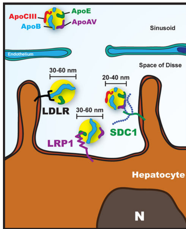
FIGURE 4. Hepatic syndecan-1 and triglyceride-rich lipoprotein clearance.
