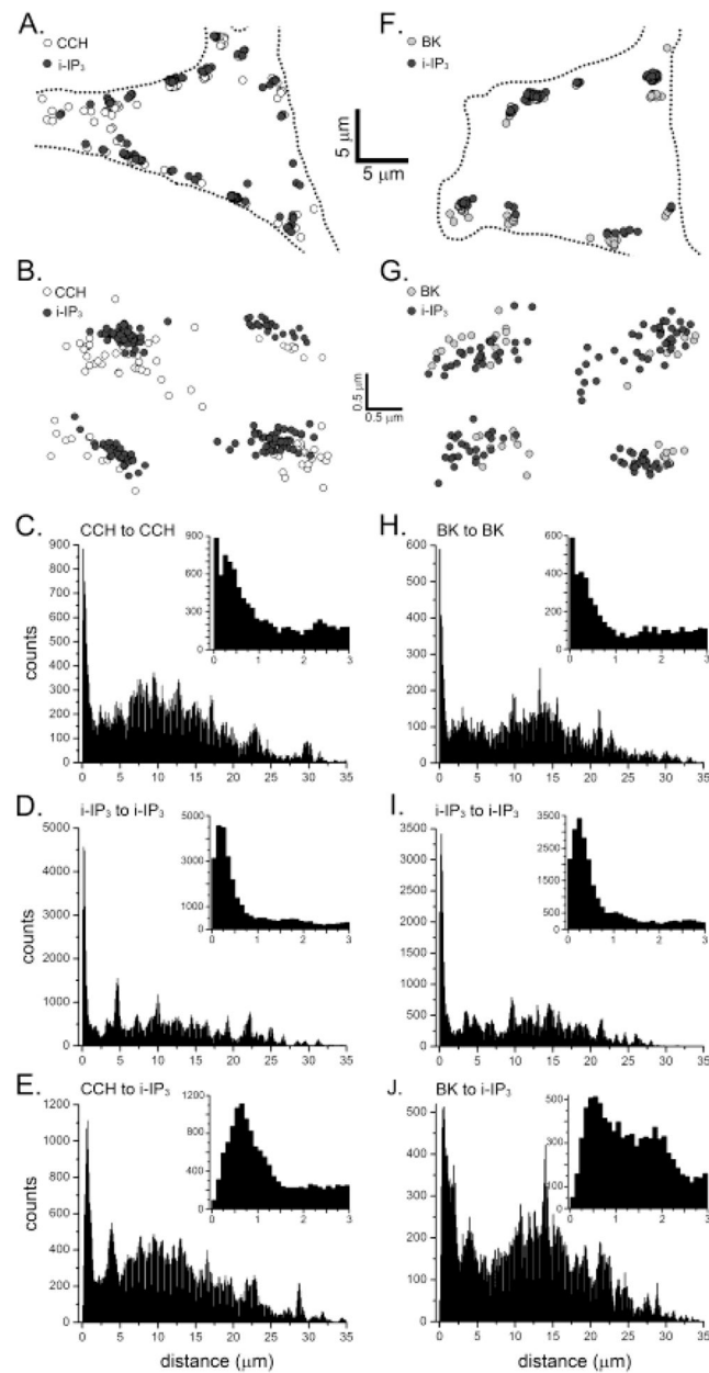
Fig. 2. GPCR agonists and \text{i-IP}_3 evoke \text{Ca}^{2+} puffs at overlapping subcellular sites. (A) The dotted outline indicates the boundary of the same cell as in Fig. 1. Open circles mark the centroid localizations of puffs evoked by CCH, and filled circles mark localizations of puffs evoked by photoreleased \text{i-IP}_3 . (B) Examples of localizations of CCH-evoked puffs (open circles) and \text{i-IP}_3 -evoked puffs (filled circles) at four sites, shown on an expanded scale. (C) Distribution of all-neighbor distances between localizations of puffs evoked by CCH. The inset in this and other panels shows the same data re-plotted on an expanded distance scale. (D) Distribution of all-neighbor distances between localizations of puffs evoked by \text{i-IP}_3 . (E) Distribution of all-neighbor distances between localizations of puffs evoked by CCH and
