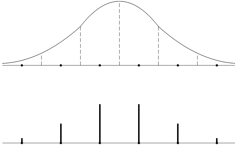
Figure 1: Approximating a continuous random variable by a discrete random variable: the support of the density function is partitioned into a finite number of intervals and each interval is represented by a value (typically the midpoint, except at the tails where the interval may be infinite) to which is assigned the probability that the random variable lies in the corresponding interval. The finer the partition and the slimmer the tail the better the approximation.
