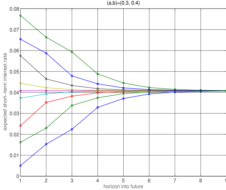
Figure 3: Forward-guidance rule: paths of expected future short-term rates for the 9 possible current inflation rates, the lower curve corresponding to -2% deflation, the upper curve to 6% inflation.
