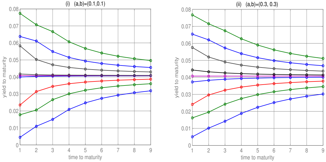
Figure 2: Term structure rule: term structures associated with the expectations matrix B in the example. In (i), (a, b) = (0.1, 0.1) ; in (ii), (a, b) = (0.3, 0.3) . Each curve represents the yield curve (r_s^\tau)_{\tau=1}^9 for a possible current inflation rate \pi_s .
