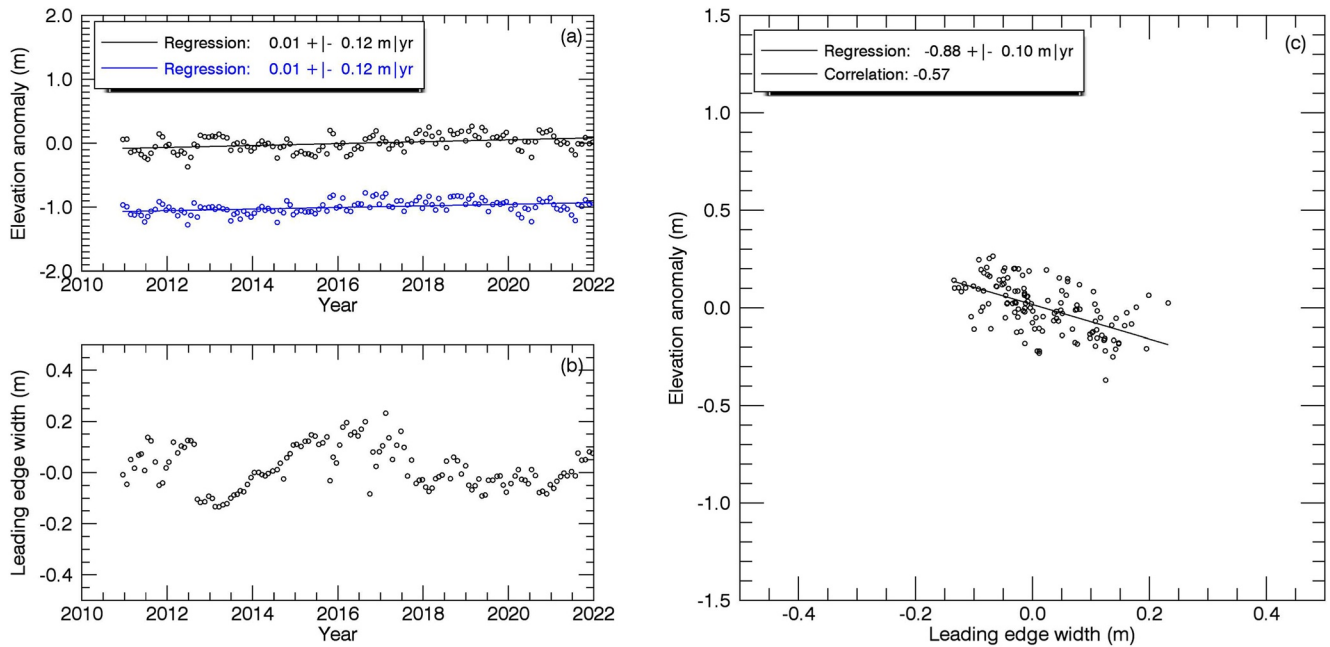
Figure 3. Effect of leading edge correction for Threshold First Maximum Retracker Algorithm (TFMRA) derived elevations shown for a 500 \text{ km}^2 area located in Northern Greenland: (a) TFMRA elevation anomaly (black) and leading edge corrected elevation anomaly (blue) (Note: for better visibility the blue graph was shifted by 1m); (b) leading edge width; (c) Linear correlation between elevation and leading edge width. The regression coefficients were used to apply the leading edge width correction.
