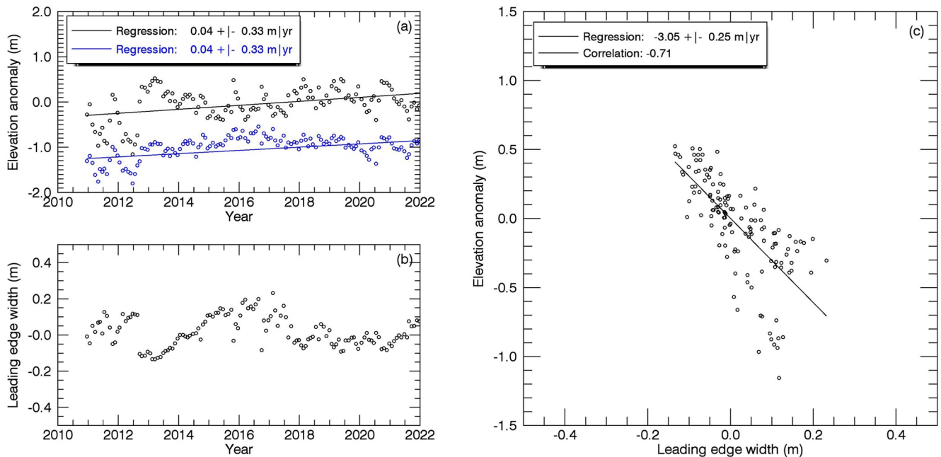
Figure 4. Effect of leading edge correction for ESA-ICE2 derived elevations shown for a 500 \text{ km}^2 area located in Northern Greenland: (a) ESA-ICE2 elevation anomaly (black) and leading edge corrected elevation anomaly (blue) (Note: for better visibility the blue graph was shifted by -1\text{m} ); (b) leading edge width; (c) Linear correlation between elevation and leading edge width. The regression coefficients were used to apply the leading edge width correction.
