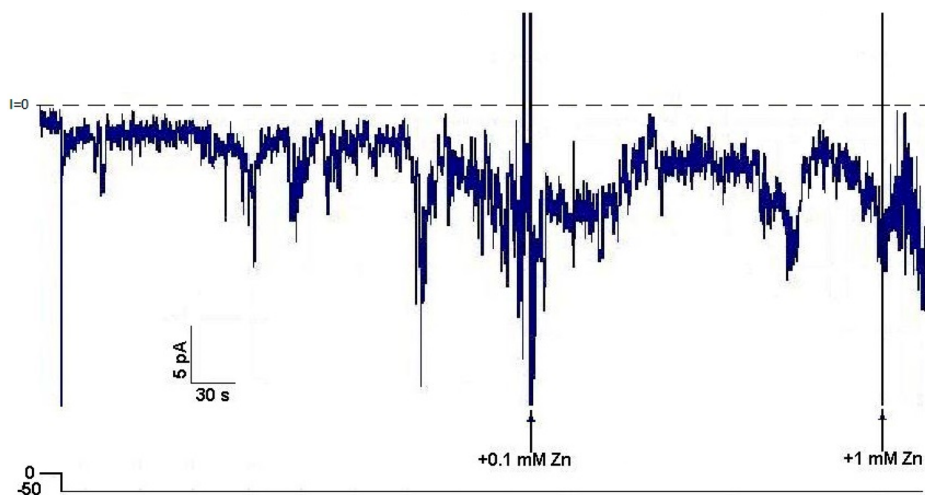
Figure 3. Unlike other amyloid beta channels, tau channels are not blocked by Zn^{2+} ions even at higher concentrations (1 mM).
