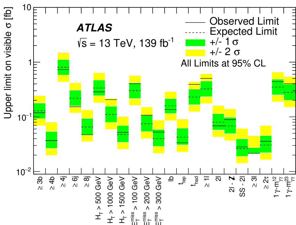
Figure 7. Observed and expected 95% CL limits on the visible cross section of BSM Higgs boson production in each signal region. The 1\sigma and 2\sigma variations of the expected limit are also shown as green and yellow bands, respectively.
