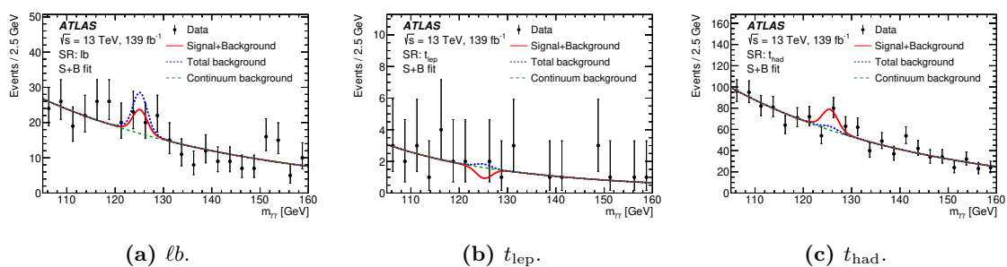
Figure 5. Diphoton mass distributions for top-quark signal regions. Data are shown together with the signal-plus-background fit. The overall fitted signal-plus-background pdf is shown as a solid red curve, the contributions from the resonant Higgs boson and continuum backgrounds are shown as a dashed blue curve, while the contributions only from the continuum backgrounds are shown as a dashed green curve. The difference between the solid red and the dashed blue curves indicates the fitted deviation from the SM expectation.
