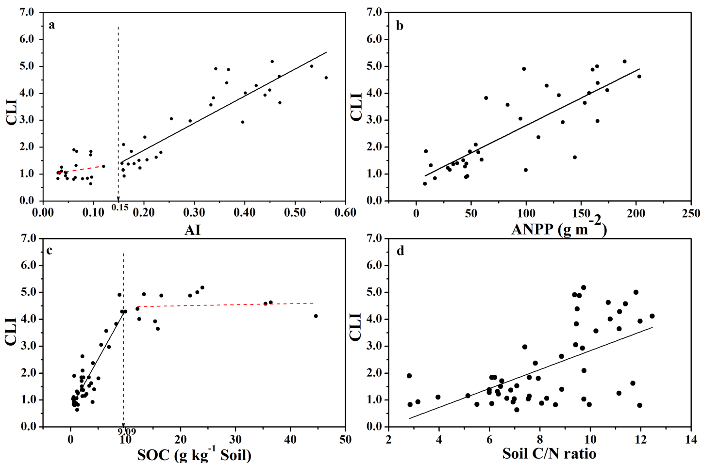
Figure 3 Changes of CLI with AI, ANPP, SOC, and soil C:N ratio for soils from the 56 locations along the sampling transect. Changes of the Carbon Limitation Index (CLI) with the aridity index (AI) (A), annual net primary productivity (ANPP) (B), soil organic carbon content (SOC) (C), and soil C:N ratio (D) for soils from the 56 locations along the sampling transect. The vertical dotted dash line indicates the AI threshold value determined by the break-point in segmented linear regression. The R^2 and P -values were obtained from linear regressions.
