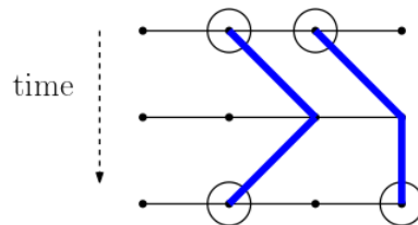
Figure 5.6: The sequence of actions x_i x_j followed by x_i^{-1} on a single rung of |\gamma\rangle , viewed as a tuple of non-intersecting paths.
