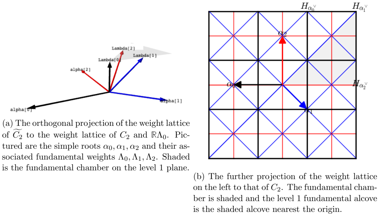
Figure 4.1: The alcove picture for C_2 , drawn using SageMath.
