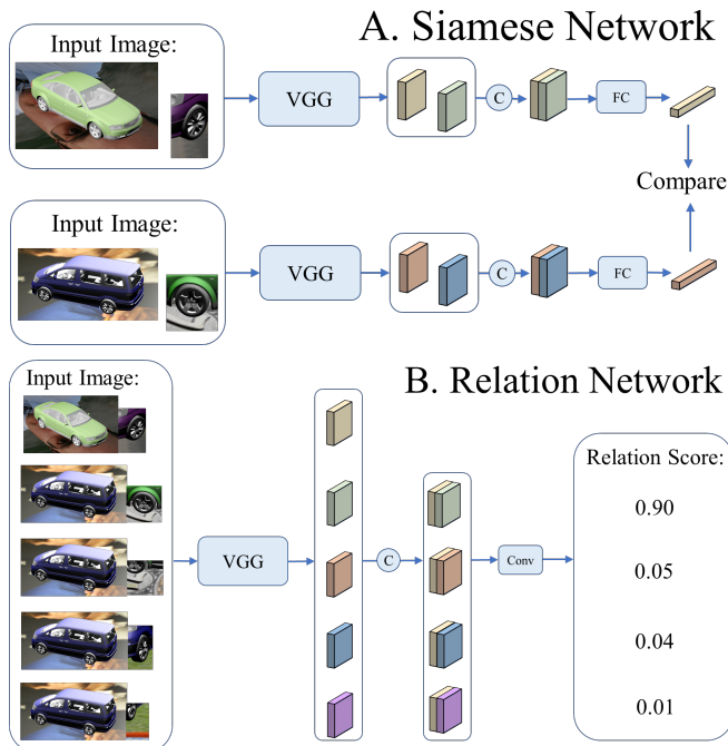
Figure 3. Siamese Network (Panel A), and Relation Network (Panel B) architectures for solving car analogy problems.
