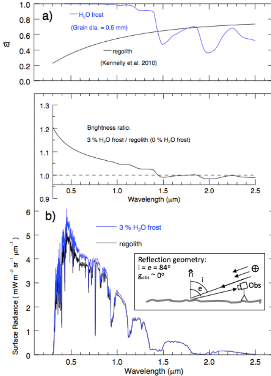
Figure 15. Simulation of Earthshine reflected from high latitude terrain, with and without a water frost component. (a) Single scattering albedo for dry regolith and water frost consisting of 0.5 mm diameter ice grains. (b) Simulated reflectance, as observed by a camera or spectrometer on the surface. Elevation angles of source (Earth) and detector are 6^\circ , with Earth located behind the sensor (inset). At visible wavelengths, water frost should be detectable using multi-wavelength (e.g. ratiometric) imaging or spectroscopy.
