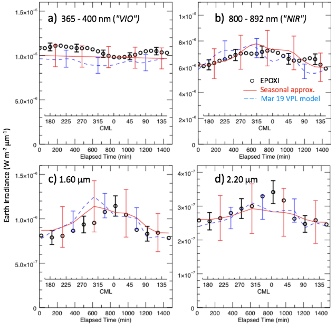
Figure 14. Comparison of the 19 March 2008 EPOXI “EarthObs1” measurements ( g = 57.5\text{--}57.8^\circ and Earth-spacecraft distance of 0.182–0.185 AU) covering one Earth rotation (black circles) with predictions of the spring season approximation, shown in red. Included for comparison is the “EarthObs1” VPL model (dashed blue lines). Panels (a) and (b) show measurements in the “VIO” and “NIR” camera channels. Panels (c) and (d) show measurements by the IR spectrometer at continuum wavelengths between \text{H}_2\text{O} bands. At 2.2\ \mu\text{m} , most of the observed modulation is due to clouds. Models and measurements are in mutual agreement, within uncertainties.
