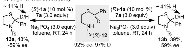
Scheme 2. Mechanistic investigations.
