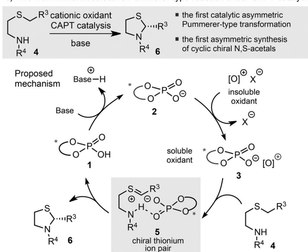
Scheme 1. Application of CAPT catalysis to the oxidative Pummerer-type C–N bond-forming reaction for the synthesis of enantioenriched N,S -acetals.
