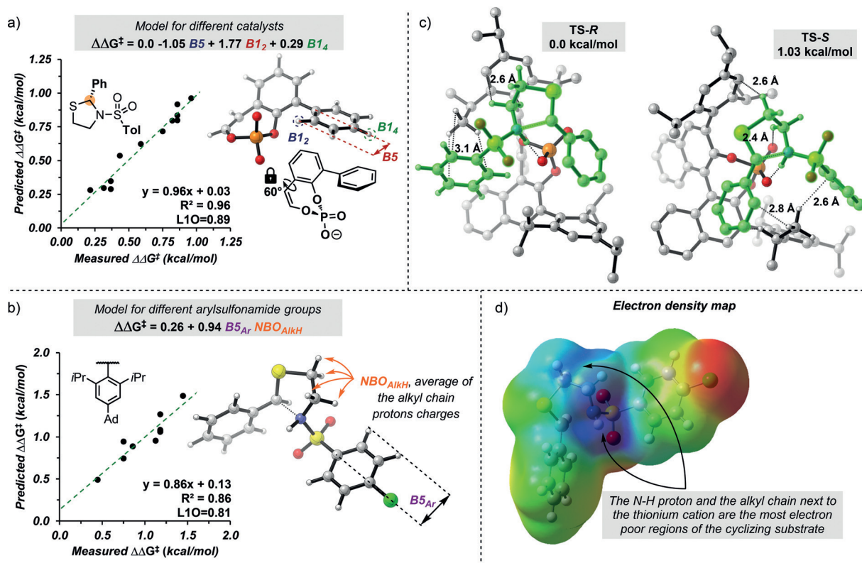
Figure 1. Multidimensional correlation analysis for the catalysts 1a–h (a) and the substrates 4a–4h (b). c) TS-R and TS-S computed at the wB97XD/6-31G(d) level of theory. wB97XD/6-311+G(2d,p)[PCM=To] energies are reported. The substrate is highlighted in green and interatomic distances are shown as dashed lines. d) Electron density map of the uncatalyzed TS of 6d .
