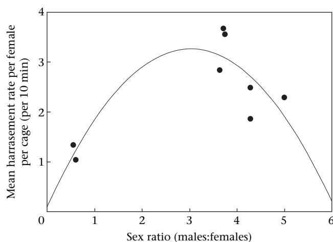
Figure 3. Effect of sex ratio (males:females) on the mean harassment rate (quadratic regression: F_{1,5} = 7.336 , R^2 = 0.746 , P = 0.0326 ). Harassment rate was highest at intermediate sex ratios.
