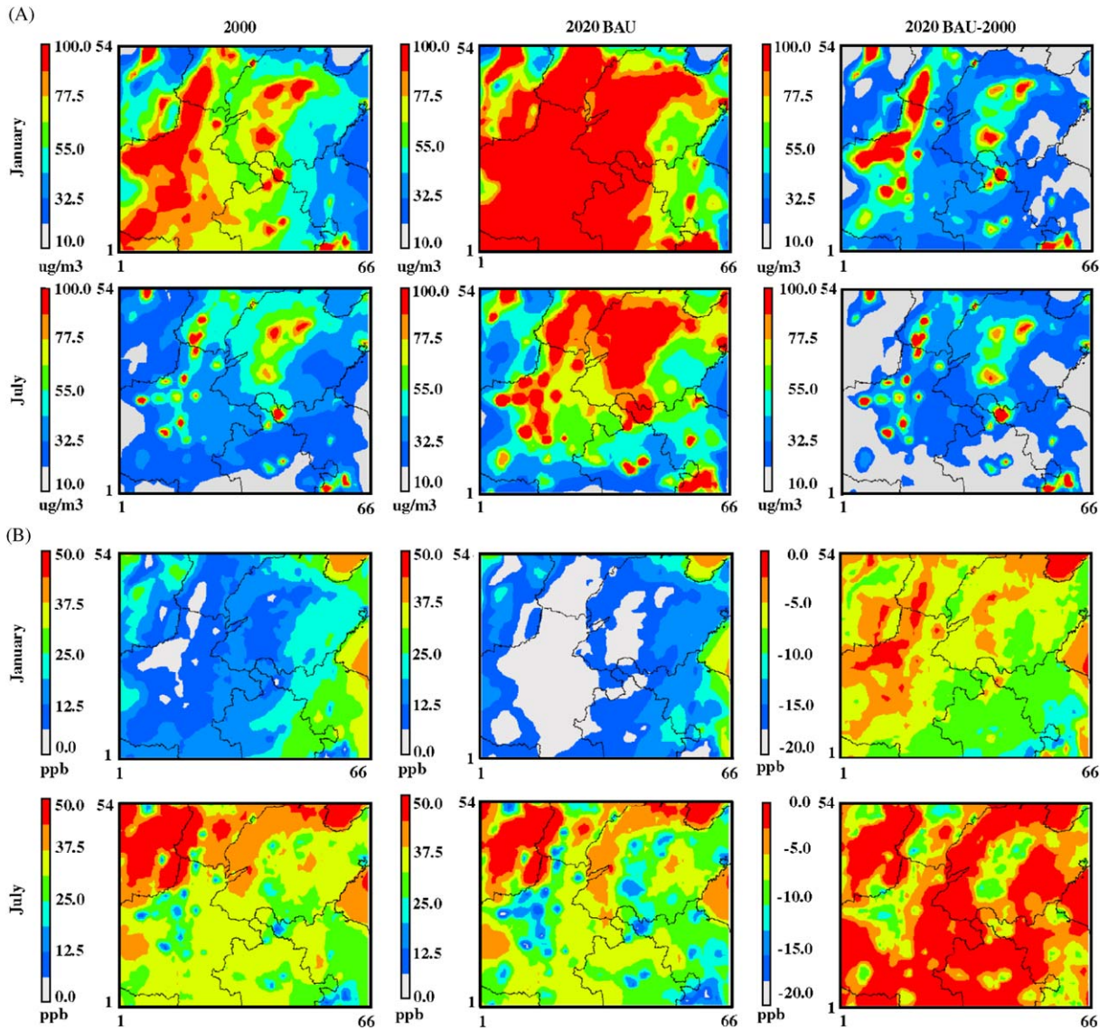
Fig. 7. Seasonal variations of surface PM_{2.5} and O_3 concentrations in 2000 and 2020 BAU. (A) PM_{2.5} and (B) O_3 .
