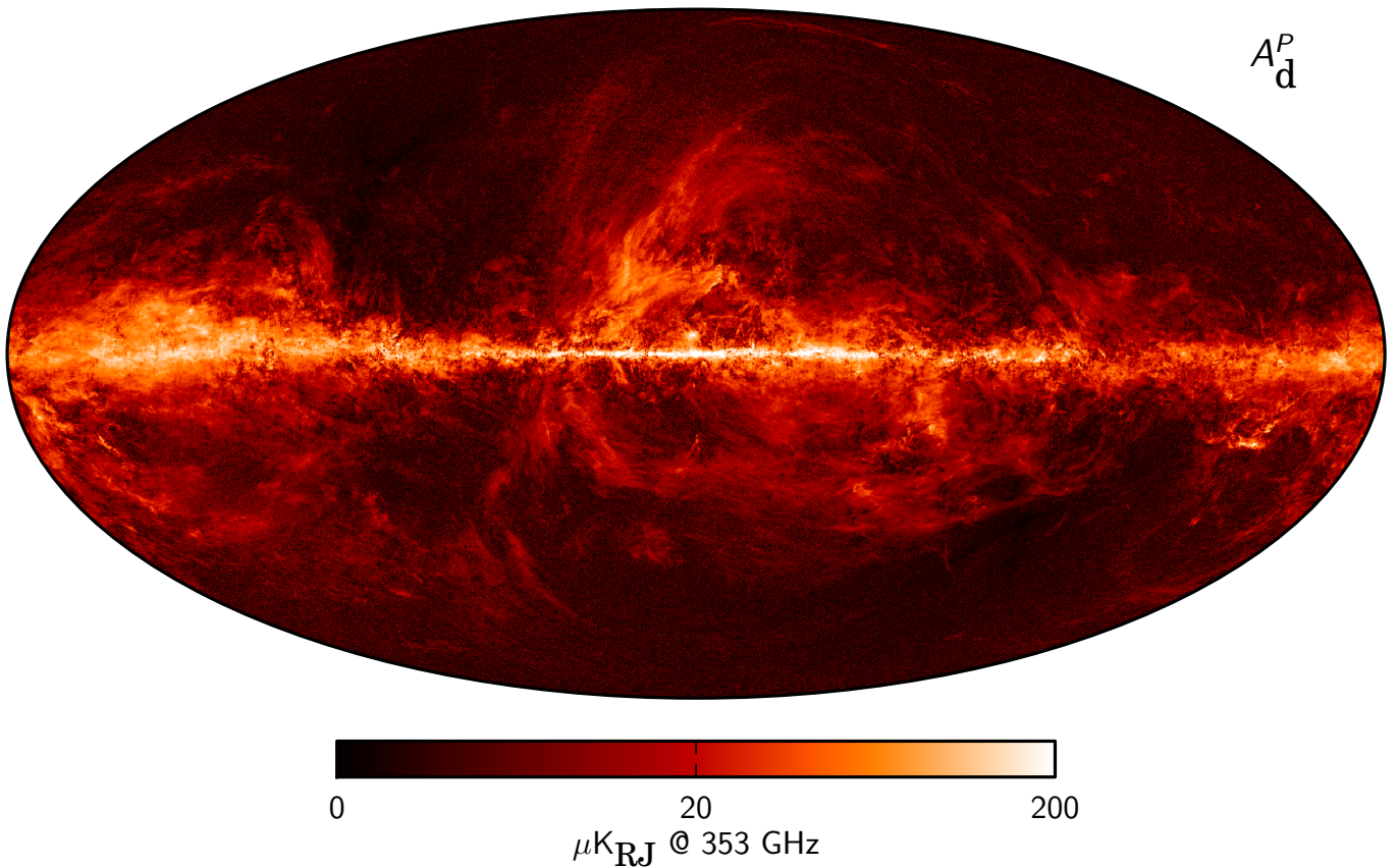
Fig. 23. Dust polarization amplitude map, P = \sqrt{Q^2 + U^2} , at 353 GHz, smoothed to an angular resolution of 10' , produced by the diffuse component separation process described in (Planck Collaboration X 2015) using Planck and WMAP data.
