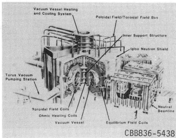
Fig. 1 An artist's conception of the Princeton Plasma Physics Laboratory TFTR experiment.
