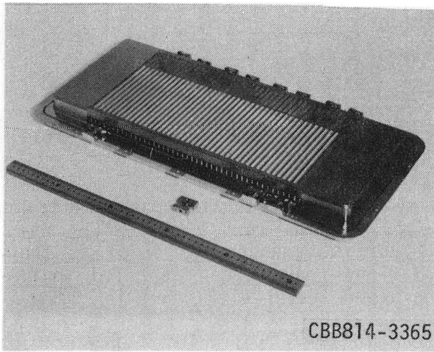
Fig. 12 "Source" electrode of the four-electrode, 80 kV, 10 cm x 40 cm long-pulse LBL accelerator.
