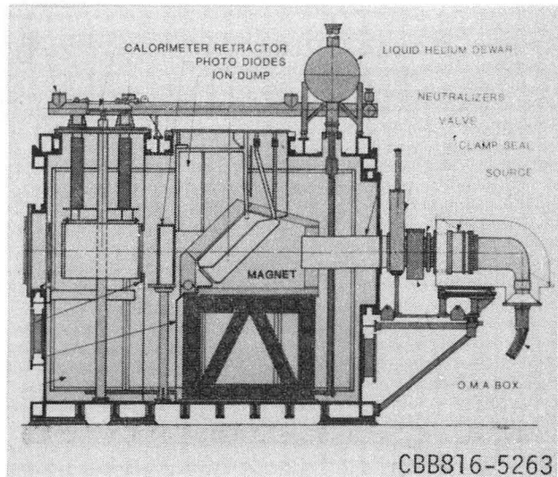
Fig. 2 Schematic of one of the positive-ion-based neutral beam systems for TFTR.
