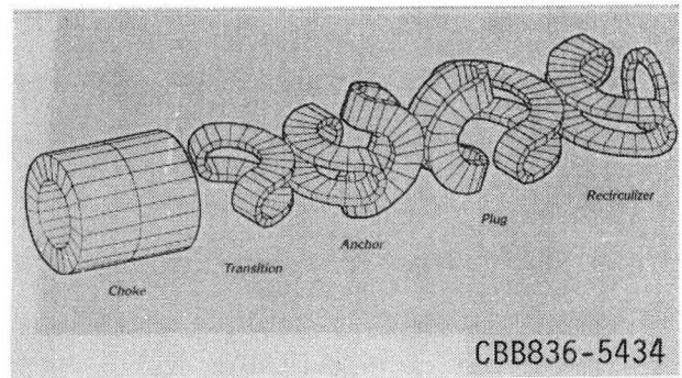
Fig. 4 Magnetic field coils in one end of the MARS tandem mirror reactor.
