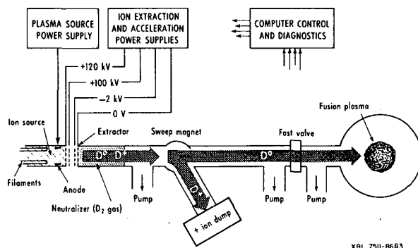
Fig. 7 Schematic of a positive-ion-based neutral beam system.
