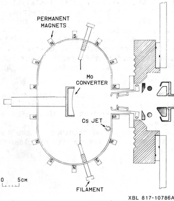
Fig. 14 Schematic diagram of LBL surface production negative-ion source.
