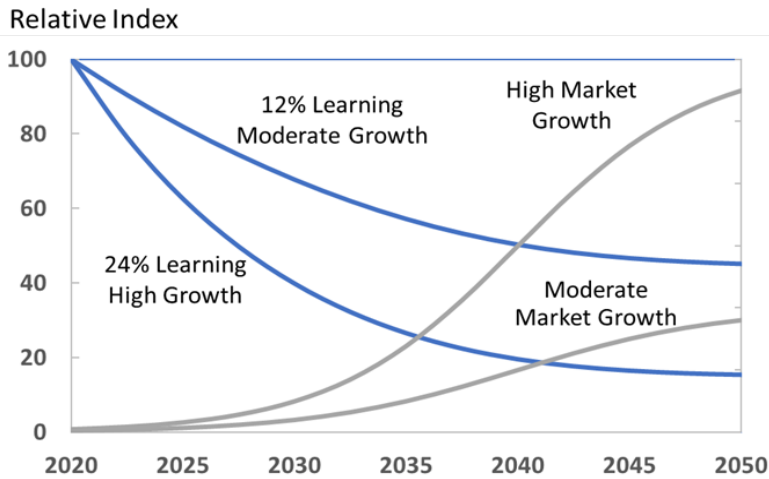
Figure 3. Learning-curve projections of electrolyzer cost evolution (blue curves) based on a lower estimate of learning rate of 12% and an upper estimate of 24% for two different market growth scenarios (grey curves).
