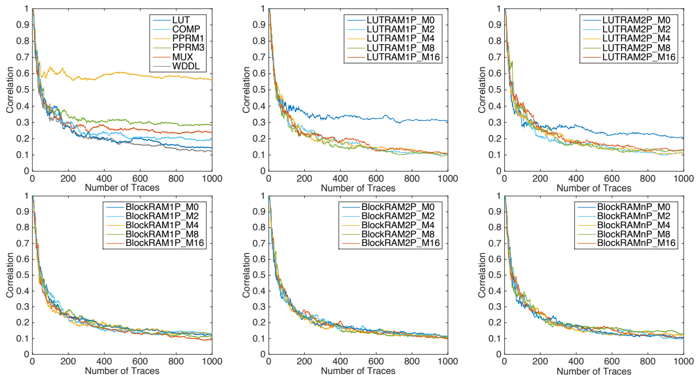
Fig. 11. Single key byte result of a first-order CPA on benchmarks with different combination of optimization strategies and the hand-written RTL benchmarks.
