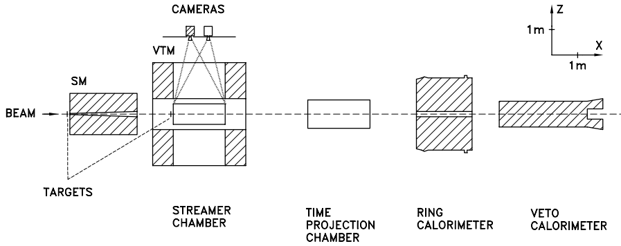
Fig. 1. Experimental setup of experiment NA35 at the CERN SPS. The target is placed either in front of the streamer chamber (SETUP I and II) or in front of the sweeper magnet SM (SETUP III)
