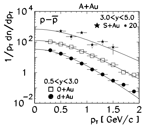
Fig. 18. Transverse momentum distributions of net protons for central d+Au, O+Au and S+Au collisions. The vertical scale is given in (\text{GeV})^{-2}
