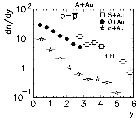
Fig. 11. Rapidity distributions of net protons ( p - \bar{p} ) for central d+Au, central O+Au and central S+Au collisions at 200 GeV/nucleon
