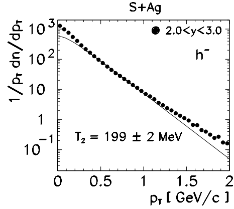
Fig. 31. Transverse momentum distribution of negatively charged hadrons produced in central S+Ag collisions. The solid line is a fit of (2) to the data in the interval 0.3 < p_T < 1.0 GeV/c. The vertical scale is given in (\text{GeV})^{-2}
