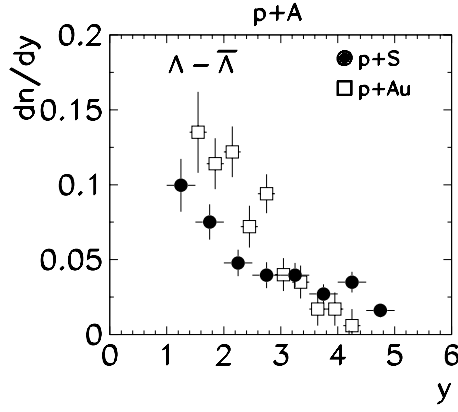
Fig. 14. Rapidity distributions of net hyperons ( \Lambda - \bar{\Lambda} ) for minimum bias p+S ( 1.0 < y < 5.0 ) and p+Au ( 1.4 < y < 4.4 ) collisions at 200 GeV/nucleon
