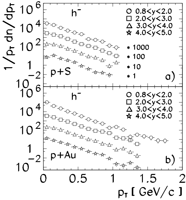
Fig. 26. Transverse momentum distributions of negatively charged hadrons produced in p+S a and p+Au b interactions for the various rapidity intervals shown. The vertical scale is given in (\text{GeV})^{-2}
