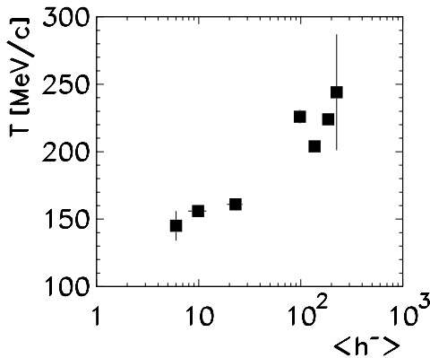
Fig. 33. 'Temperature' of net protons for p-nucleus, deuteron-nucleus and central nucleus-nucleus collisions as a function of the average multiplicity of negatively charged hadrons
