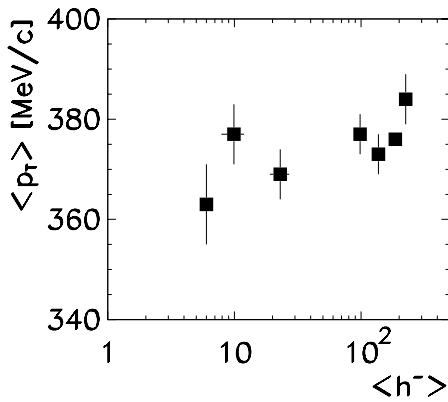
Fig. 32. Average transverse momentum in 2 < y < 3 of negatively charged hadrons produced in p-nucleus, deuteron-nucleus and nucleus-nucleus collisions as a function of the average multiplicity
