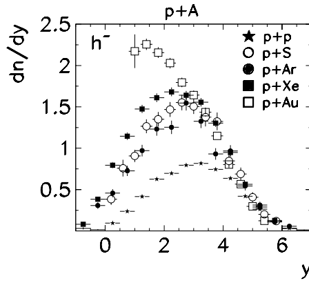
Fig. 21. Rapidity distributions of negatively charged hadrons produced in minimum bias p+p, p+S, p+Ar, p+Xe and p+Au collisions [36]. Note that the rapidity distribution for p+S collisions is higher than for p+Ar interactions due to different trigger conditions and event selections
