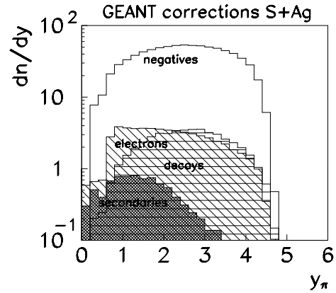
Fig. 8. Composition of a measured rapidity spectrum of negatively charged particles, based on a tuned event generator (FRITIOF) and a GEANT simulation
