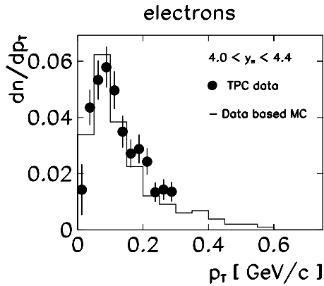
Fig. 6. Transverse momentum spectrum of conversion electrons in central S+S collisions measured and identified in the TPC in the pion rapidity range 4.0 \leq y \leq 4.4 compared to a calculated spectrum based on the measurement of negatively charged hadrons (see text for details). The vertical scale is given in (\text{GeV}/c)^{-1}
