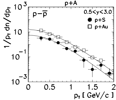
Fig. 17. Transverse momentum distributions of net protons for minimum bias p+S and p+Au collisions. The vertical scale is given in (\text{GeV})^{-2}
