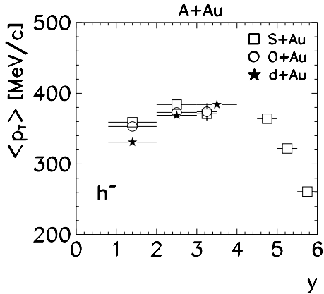
Fig. 30. Mean transverse momentum of negatively charged hadrons produced in d+Au, central O+Au and S+Au collisions as a function of rapidity
