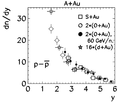
Fig. 12. Scaled rapidity distributions of net protons for central 16·(d+Au), central 2·(O+Au) and central S+Au collisions. For the case of the 60 GeV/nucleon data the rapidities are scaled by the ratio of the beam rapidity relative to that of 200 GeV/nucleon
