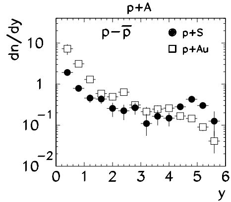
Fig. 10. Rapidity distributions of net protons ( p - \bar{p} ) for minimum bias p+S and p+Au collisions at 200 GeV/nucleon
