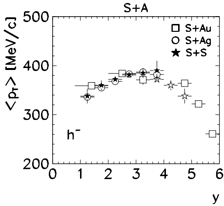
Fig. 29. Mean transverse momentum of negatively charged hadrons produced in central S+S, S+Ag and S+Au collisions as a function of rapidity. The open stars are S+S data reflected at y = 3
