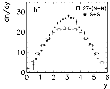
Fig. 24. Rapidity distributions of negatively charged hadrons produced in central S-S collisions and in minimum bias nucleon-nucleon interactions (scaled by the ratio of participant nucleons)
