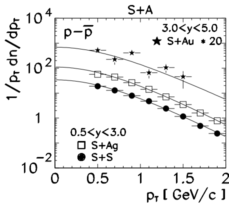
Fig. 19. Transverse momentum distributions of net protons for central S+S, S+Ag and S+Au collisions. The vertical scale is given in (\text{GeV})^{-2}
