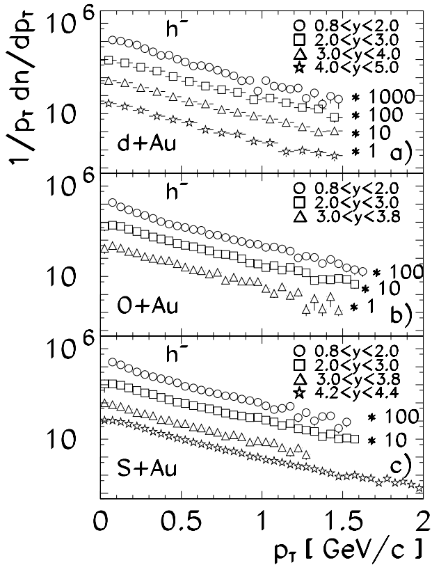
Fig. 27. Transverse momentum distribution of negatively charged hadrons produced in central d+Au a, central O+Au b and central S+Au c collisions at different rapidities. The vertical scale is given in (\text{GeV})^{-2}
