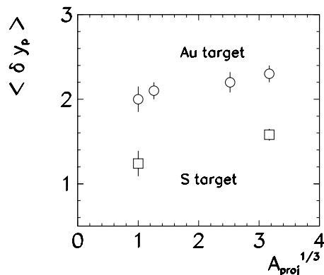
Fig. 16. Average rapidity loss (mean rapidity shift) of net projectile protons for various projectiles incident on sulphur and gold targets at 200 GeV per nucleon
