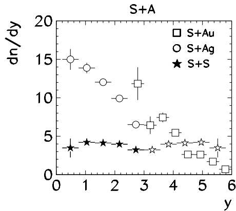
Fig. 13. Rapidity distributions of net protons ( p - \bar{p} ) for various central S-nucleus collisions at 200 GeV/nucleon
