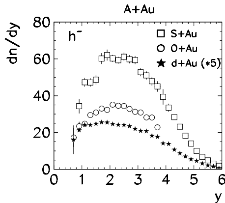
Fig. 22. Rapidity distributions of negatively charged hadrons produced in central d+Au, O+Au and S+Au collisions
