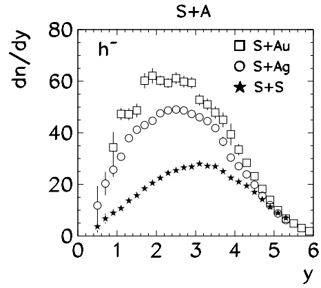
Fig. 23. Rapidity distributions of negatively charged hadrons produced in central S-nucleus collisions
