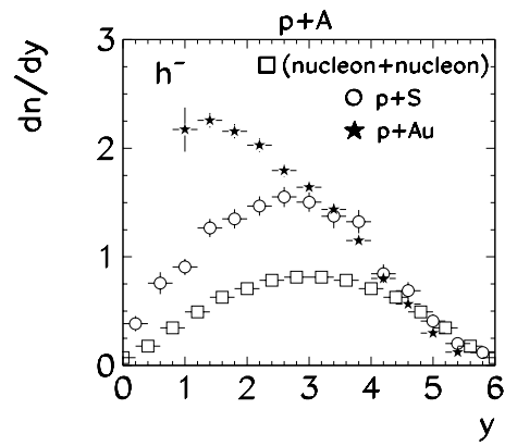
Fig. 20. Rapidity distributions of negatively charged hadrons produced in minimum bias nucleon–nucleon, p+S and p+Au collisions
