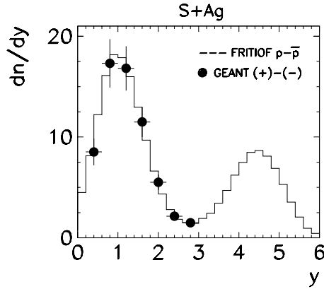
Fig. 9. Simulated rapidity distributions of net protons ( p - \bar{p} ) and of reconstructed net protons deduced from the charge excess after all corrections for central S+Ag collisions
