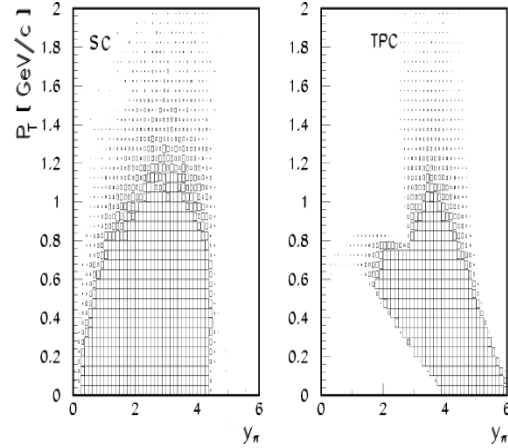
Fig. 3. Acceptance of the two large-volume tracking detectors, the streamer chamber (left) and TPC (right) for SETUP II, illustrated by the phase-space population of negatively charged hadrons in a typical heavy ion collision
