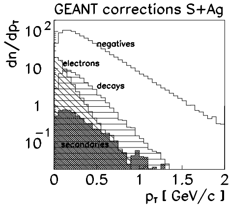
Fig. 7. Composition of a measured transverse momentum spectrum of negatively charged particles, based on a tuned event generator (FRITIOF) and a GEANT simulation. The vertical scale is given in (\text{GeV}/c)^{-1}
