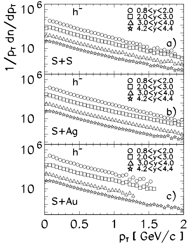
Fig. 28. Transverse momentum distribution of negatively charged hadrons produced in central S+S a, S+Ag b and S+Au c collisions at different rapidities. The vertical scale is given in (\text{GeV})^{-2}
