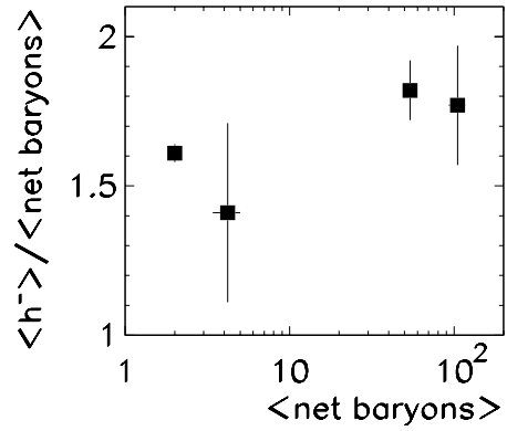
Fig. 25. Average total multiplicity of negatively charged hadrons per net baryon produced in minimum bias nucleon–nucleon, p+S, central S+S and S+Ag collisions as a function of the number of net baryons
