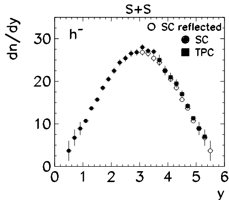
Fig. 5. Rapidity distributions of negatively charged hadrons produced in central S+S collisions, measured in the streamer chamber (SETUP II) and reflected around y_{cm} = 3 , and in the TPC
