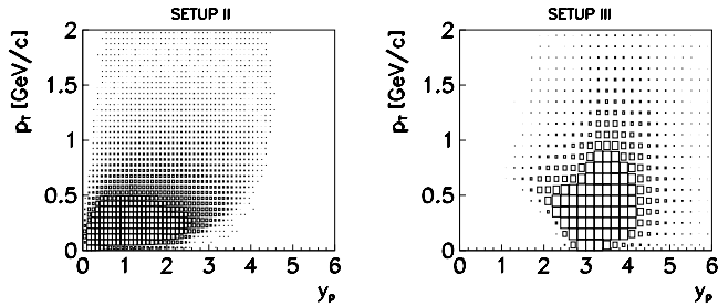
Fig. 2. Acceptance of the streamer chamber in configuration SETUP II (left) and SETUP III (right) for protons, illustrated by the phase space population in a typical heavy ion collision. Note the forward acceptance of SETUP III
