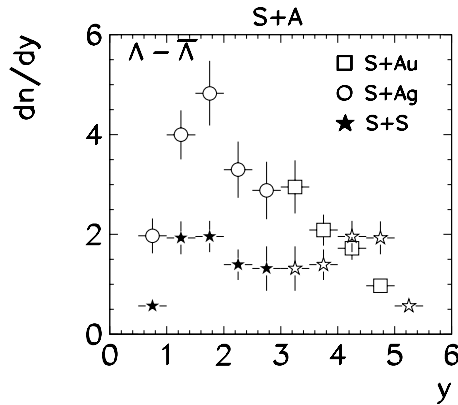
Fig. 15. Rapidity distributions of net hyperons ( \Lambda - \bar{\Lambda} ) for central S+S ( 0.5 < y < 3.0 ), S+Ag ( 0.5 < y < 3.0 ) and S+Au ( 3.0 < y < 5.0 ) collisions at 200 GeV/nucleon. The solid stars are measured S+S data, the open stars are reflected at y = y_{cm}
