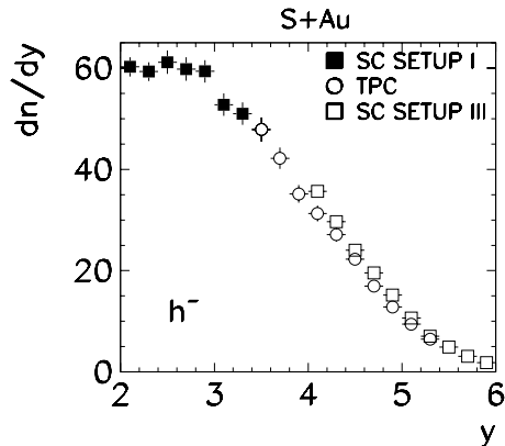
Fig. 4. Rapidity distributions of negatively charged hadrons (pion mass assumed) produced in central S+Au collisions, measured in the streamer chamber (configurations SETUP I and SETUP III) and in the TPC
