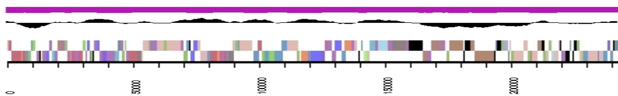
Figure 9. Graphical map of the genome of Rhizobium leguminosarum bv. trifolii strain SRDI565 (7.7). From bottom to the top of each scaffold: Genes on forward strand (color by COG categories as denoted by the IMG platform), Genes on reverse strand (color by COG categories), RNA genes (tRNAs green, sRNAs red, other RNAs black), GC content, GC skew.
