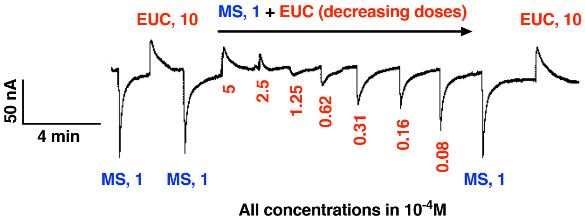
Figure S4. Eucalyptol (EUC)-elicited, dose-dependent inhibition of responses of CquiOR32-Orco-expressing oocytes to methyl salicylate (MS). Continuous trace from the same oocyte.
