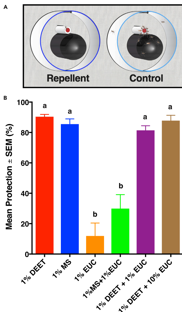
Figure 11. Effect of Eucalyptol on Methyl Salicylate-Elicited Repellency
