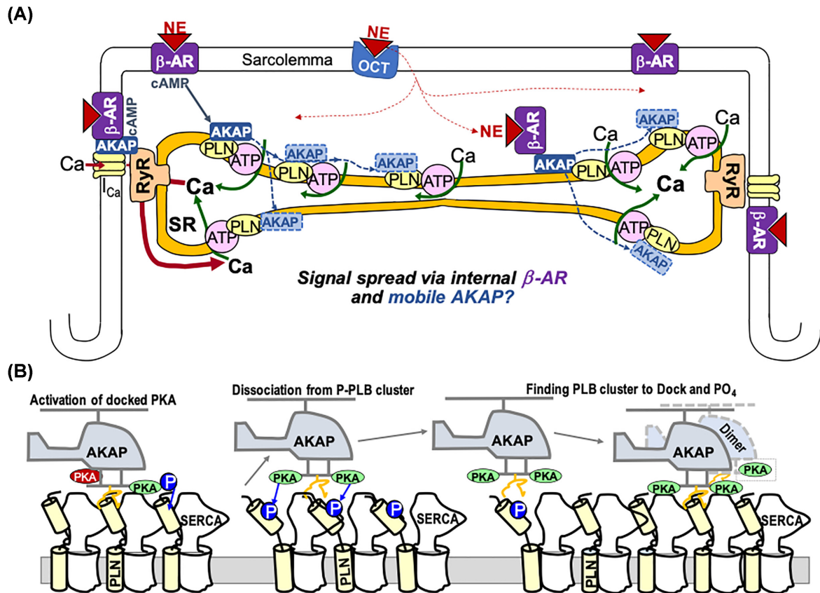
Figure 9. Working hypothesis for \beta -AR signal spread in myocytes. (A) Norepinephrine activates \beta -AR, which raises cAMP and activates myocyte PKA. Norepinephrine can enter via OCT, diffuse and activate intracellular \beta -ARs, contributing to PLN phosphorylation and acceleration of SR Ca uptake. AKAP7 \gamma may shuttle active PKA along the surface of the SR membrane. Together these two mechanisms may facilitate rapid spatial \beta -AR signaling to SR Ca uptake. (B) AKAP7 \gamma binds to PLN near its PKA phosphorylation site (Left). When inactive PKA (red) binds cAMP and becomes activated (green), it can phosphorylate nearby PLN (left to center). When all local PLN is phosphorylated (center), it reduces PLN-AKAP7 \gamma affinity, facilitating dissociation. Active PKA-AKAP7 \gamma can diffuse (hover) along the SR surface and quickly finds other clusters of unphosphorylated PLN to bind to and phosphorylate. AKAP7 \gamma dimerization may help restrict this diffusion to the SR surface if only one monomer is released from the PLN at a time (hand-over-hand). Thus, AKAP7 \gamma moves along the SR surface, rapidly phosphorylating PLN.
