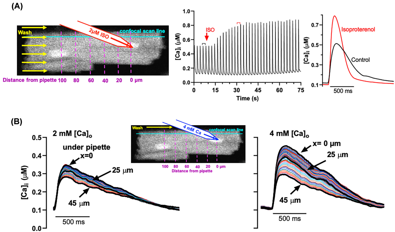
Figure 2. (A) Experimental protocol. The pipette was loaded with 2 \mu\text{M} ISO. A representative time course of Ca transients is shown at right. Upon local ISO application, peak [\text{Ca}]_i grew progressively higher and rate of [\text{Ca}]_i transient decline accelerated until a new steady-state was reached. (B) Typical steady-state [\text{Ca}]_i transients from an experiment where the pipette was loaded with 4 mM Ca. Steady-state [\text{Ca}]_i at the indicated distances before high Ca addition are on the left. After Ca addition to the end of the cell (right), the peak steady-state [\text{Ca}]_i increased most strongly underneath the pipette. The increase in peak [\text{Ca}]_i along the scan line became progressively lower the farther upstream from the pipette that the measurement was taken.
